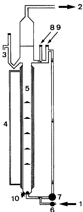
Fig. 1. The anaerobic fluidized bed reactor. Medium and suspended cells were pumped upwards through a water-jacketed vertical cylinder [5] (working volume, 3 l) on which was mounted an expansion head. The liquid passed a pH-stat set at pH 7.2 (inlet for 2 M NaOH [8]; electrode [9]) and was driven through the system by a pump [7]. The temperature was maintained at 35°C by a thermostat [4]. The culture was largely immobilized on activated charcoal (initial packed volume, 0.4 l). Medium with chloroacetate as the sole carbon source was pumped [6] from a 5-l anaerobic reservoir [1] into the system at 21 ml/h. The volume was maintained constant by an overflow [3] and gaseous products vented at [2]. The system had one sampling port [10] from which portions of the fluidized bed could be withdrawn
