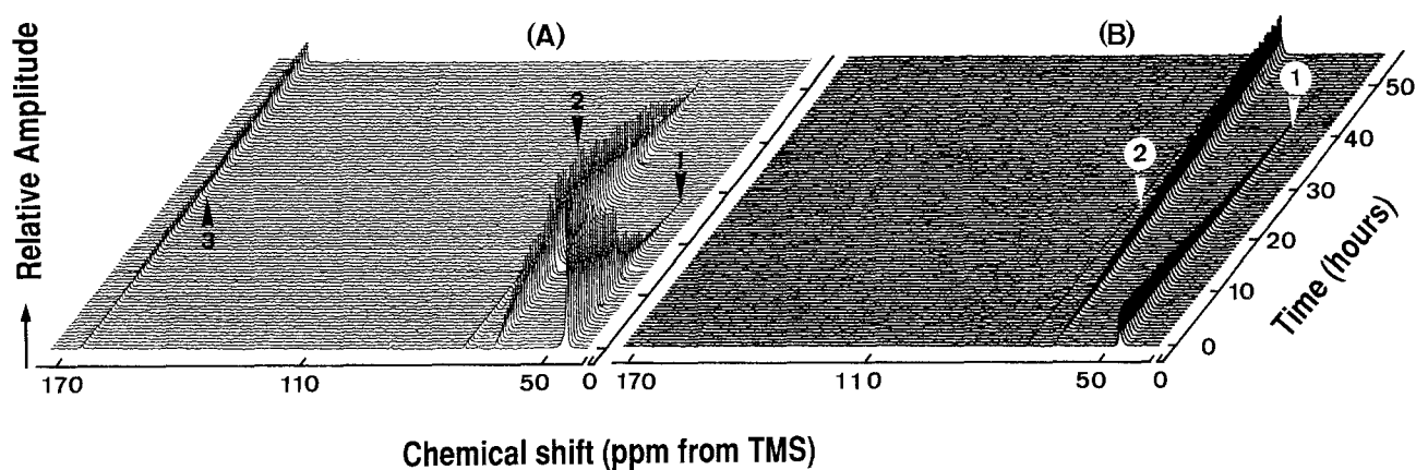
Fig. 3 A, B. Kinetics of the transformation of [2- 13 C]chloroacetate to products by the methanogenic mixed culture immobilized on charcoal. The vessel containing the biological reaction mixture was mounted in a 13 C-NMR spectrometer and spectra were taken at intervals and plotted as pseudo-3-dimensional graphs. The chemical shifts (ppm) of standards (the 13 C-component of authentic materials) measured under identical conditions, which agreed with literature data (Pretsch et al. 1976), identified the signals as [2- 13 C]chloroacetate [48.8 ppm; marked 1 in (A) + (B)], [2- 13 C]glycolate [67.4 ppm; marked 2 in (A) + (B)] and 13 CO 3 2- [168.3 ppm; marked 3 in (A)]. Two representative experiments are shown: (A), under strictly anaerobic conditions (9 mM chloroacetate); (B) under aerobic conditions (3 mM chloroacetate)
