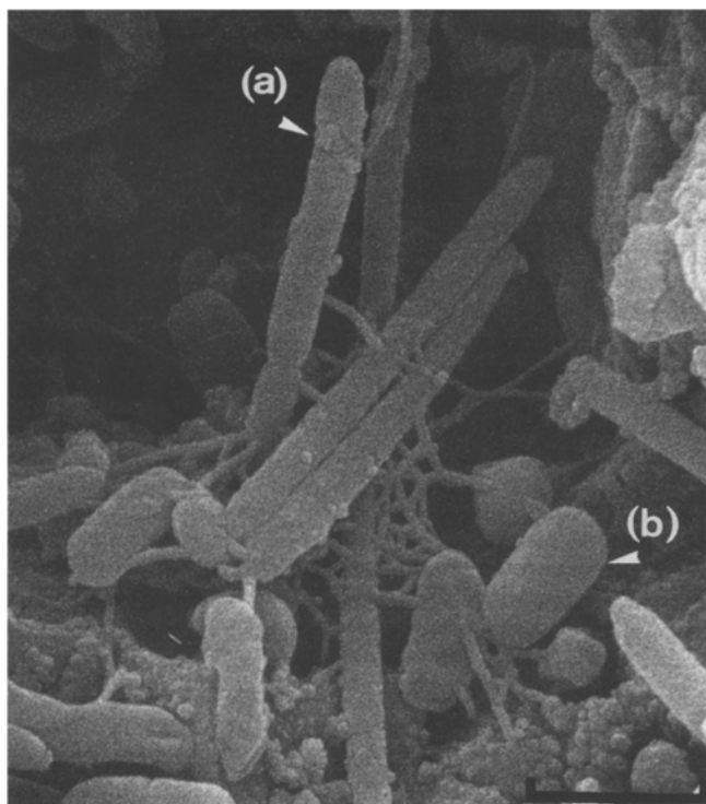
Fig. 2. Electron micrograph of the methanogenic mixed culture immobilized on charcoal. Two predominant, morphologically different bacteria were observed: (a) a long rod ( 3 \times 0.3 \mu\text{m} ), presumed to be a methanogen because of its F420 autofluorescence and (b) a short ( 0.9 \times 0.6 \mu\text{m} ), non-methanogenic organism. The bar represents 1 \mu\text{m}
