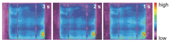
Figure 6: Fast iLIT measurements of an EFG solar cell (same conditions as for the measurements shown in Figure 4).
