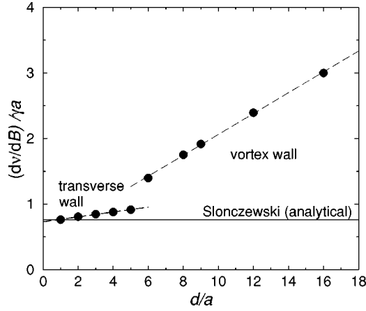
FIG. 3. Domain wall mobility vs diameter of cylindrical systems. The model parameters are \omega/J=0.003 , D_e/J=0.1 , \alpha=1 . The constant line corresponds to Eq. (3); the dashed lines are guides to the eye. Error bars are smaller than the symbol size.
