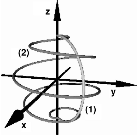
FIG. 4. Two different paths for the reversal of a spin. While (2) is dominated by precession, as in a transverse wall, path (1) is restricted to one plane as in a vortex wall.
