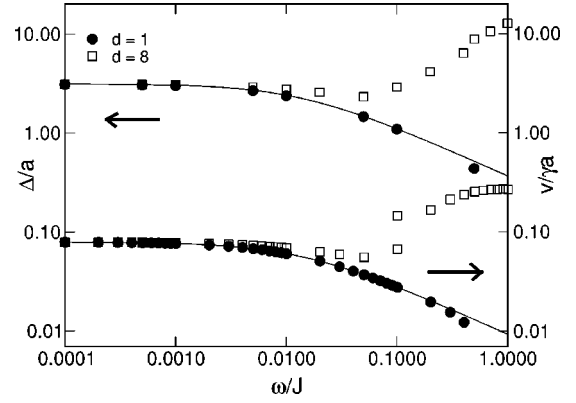
FIG. 2. Domain wall velocity and domain wall width vs dipolar coupling for a spin chain and a cylindrical system, respectively. D_e/J=0.05 , \mu_s B/J=0.05 , \alpha=1 . The solid lines correspond to Eqs. (4) and (3); error bars are smaller than the symbol size.
