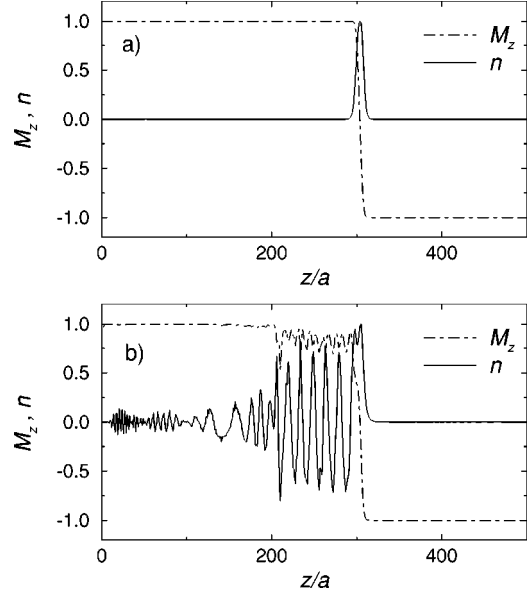
FIG. 6. Profiles and winding numbers of moving vortex walls in (a) the high-damping limit ( \alpha=1 ) and (b) the low-damping limit ( \alpha=0 ). d=8 , \omega/J=0.2 , D_e/J=0.05 , \mu_s B/J=0.1 .
