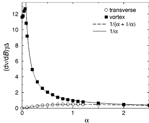
FIG. 5. Reduced domain wall mobility vs damping constant. The model parameters are \omega/J=0.01 (transverse wall) and \omega/J=0.7 (vortex wall), respectively, D_e/J=0.05 , \mu_s B/J=0.05 , d=4 . Error bars are smaller than the symbol size.
