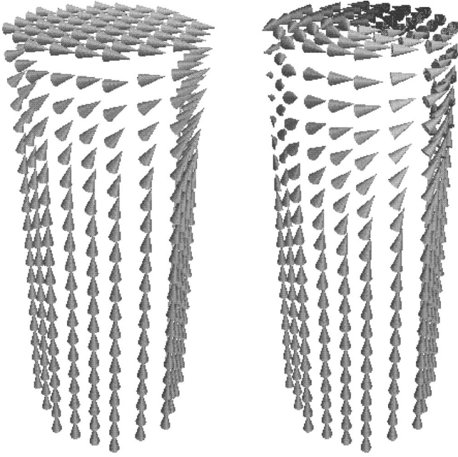
FIG. 1. Snapshots of a transverse (left, \omega/J=0.003 ) and a vortex (right, \omega/J=0.2 ) wall. The diameter d=8 is kept constant while the exchange length of the system is varied. Shown is only a part of the system below the current wall position. D_e/J=0.05 .
