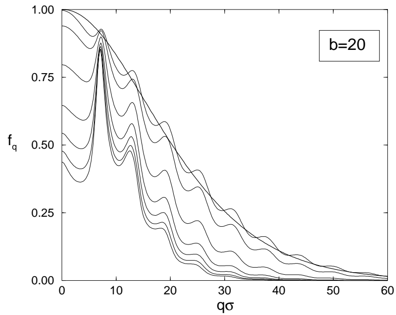
Figure 3. HCAY critical coherent non-ergodicity parameters f_q for b = 20 as in figure 2. The K -values, incremented by 2, run from bottom to top from 0 to 12. The asymptotic prediction from equation (4) is shown as the bold curve.
