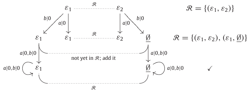
Fig. 5. Bisimulation construction.
