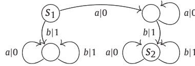
Fig. 6. Mealy machine: s_1 \sim s_2 .
