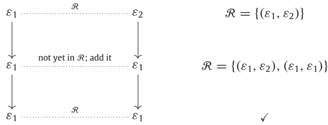
Fig. 1. Bisimulation construction.
