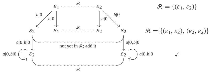
Fig. 4. Bisimulation construction.
