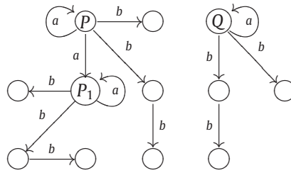
Fig. 8. Nondeterministic processes: Q \sim P .
