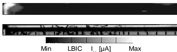
Figure 6: Magnified part of thermogram (top) and high resolution LBIC map (980 nm) (bottom) of the wafer which was edge isolated by sawing trenches in the back side after the printing. In the LBIC map the positive effect of the emitter going around the edge of the cell is visible (bright area, top) compared to the rest of the wafer (less bright, bottom). The bad stripe in between (black) results from the trench in the back side. In addition the shunt in the corner of the wafer is visible in both measurements.
