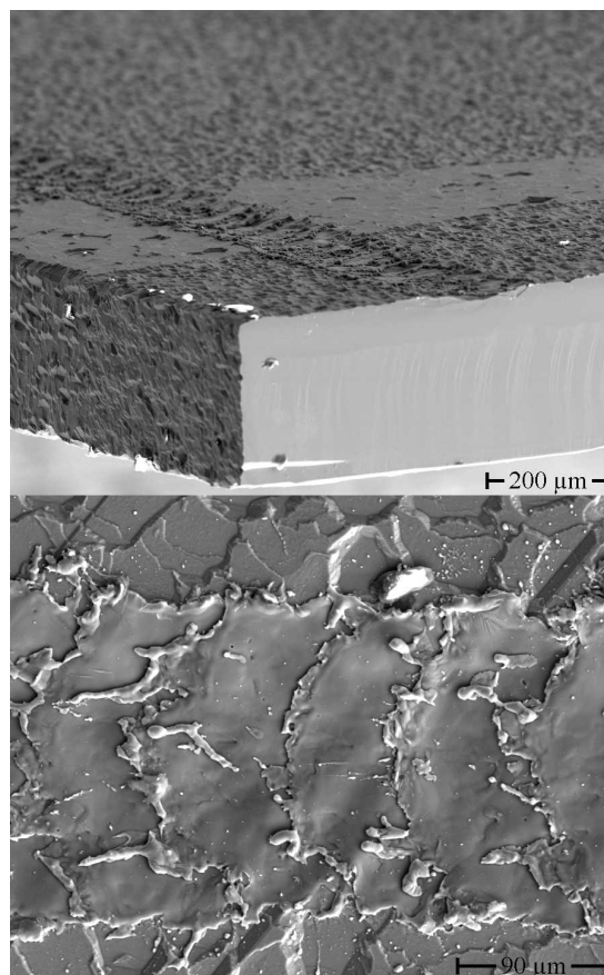
Figure 1: Electron microscope pictures of a laser trench. On the lower picture the trench is seen from top. The recrystallized structures of the laser spots can be seen. Laser was moving from left to right.
