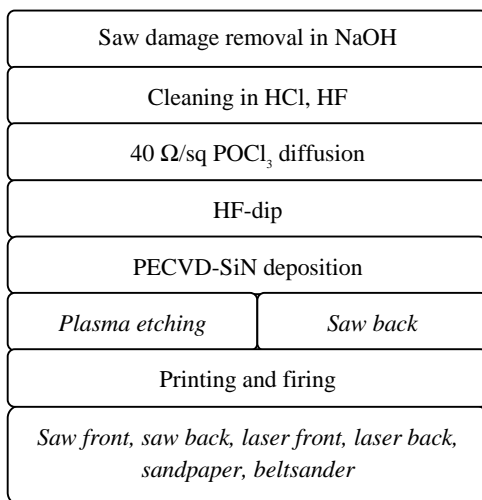
Figure 2: Processing sequence of the solar cells. The edge isolation steps are written in italics.
