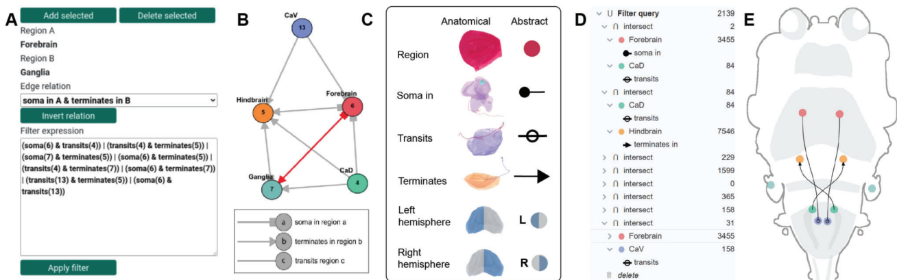
Fig. 3. Design prototype and proposed solution. A: Initial visual interface for specifying query expressions. B: First prototype for displaying the constructed neural circuit as abstract 2D graph. C: Anatomical units and their abstract representation. D: New query builder (Section V-A1) for interactive query building. E: Circuit viewer (Section V-C1) for intuitive visualization of neural circuits.
