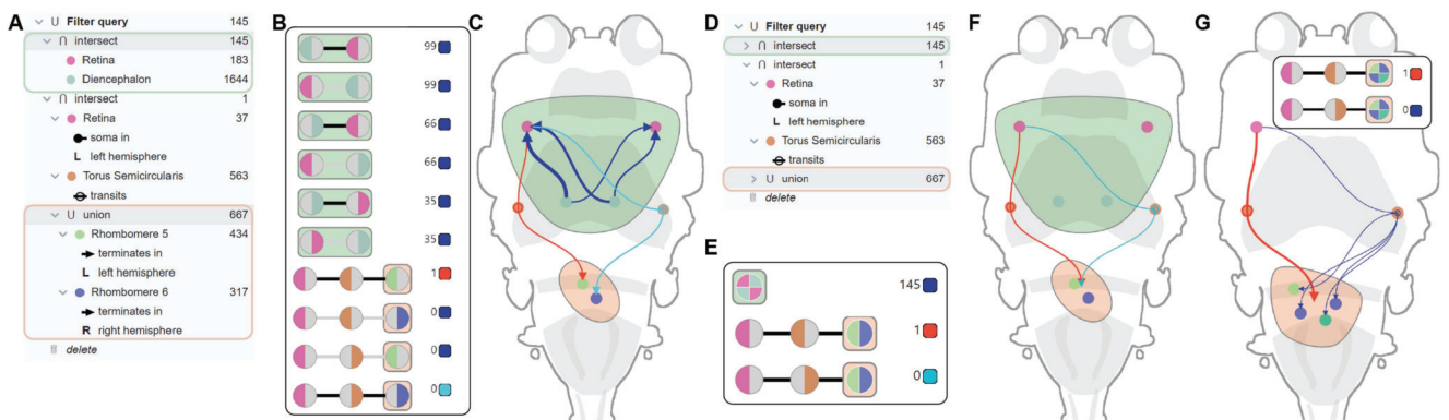
Fig. 6. Visual components (Section V). A : Query builder (Section V-A1), showing the example query; the selected sub-queries are highlighted by green and orange bounding boxes, respectively. B : Pathway browser (Section V-B1), displaying the list of possible connections realizing the example query. C : Circuit viewer (Section V-C1), showing the realized neural circuits and regions corresponding to selected sub-queries enclosed by an envelope. The thickness of the blue connections encodes to number of neurons. D : Query builder (Section V-A1), showing the collapsed sub-queries. E : Pathway browser (Section V-B1), displaying the list of partially aggregated pathways. F : Circuit viewer (Section V-C1), showing the pathways as partially aggregated edges. G : Circuit viewer (Section V-C1), depicting two different selection modes for partially aggregated pathways. In the default mode, the links to all regions in the corresponding set are shown, e.g., pathways in the right hemisphere. Alternatively, an aggregated representation of pathways, e.g., the red line leading to the orange region, is displayed as an aggregated edge.
