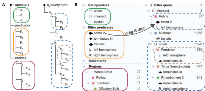
Fig. 5. Query builder . A : Set operators, filter predicates, and biological entities (left tree) are used to construct a filter query (right tree). B : In our application, filter predicates describe spatial attributes of neurons in relation to regions. The user builds a query by dragging operators, spatial predicates and regions into the query tree.
