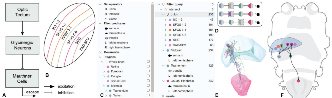
Fig. 1. A: Graphical illustration of a circuit hypothesis concerning inhibiting escape behavior in larval zebrafish, described in detail in case study 1 (Section VI-C). B: Layers of the optic tectum used in hypothesis 2 of case study 1 (Section VI-C). C: Generation of a query for searching groups of neurons, using the query builder (Section V-A1). D: Listing of possible pathways using the pathway browser (Section V-B1). E: 3D viewer showing the morphology of neurons matching the filter criteria (Section V-C2). F: Visualization of a neuron circuit using the circuit viewer (Section V-C1).
