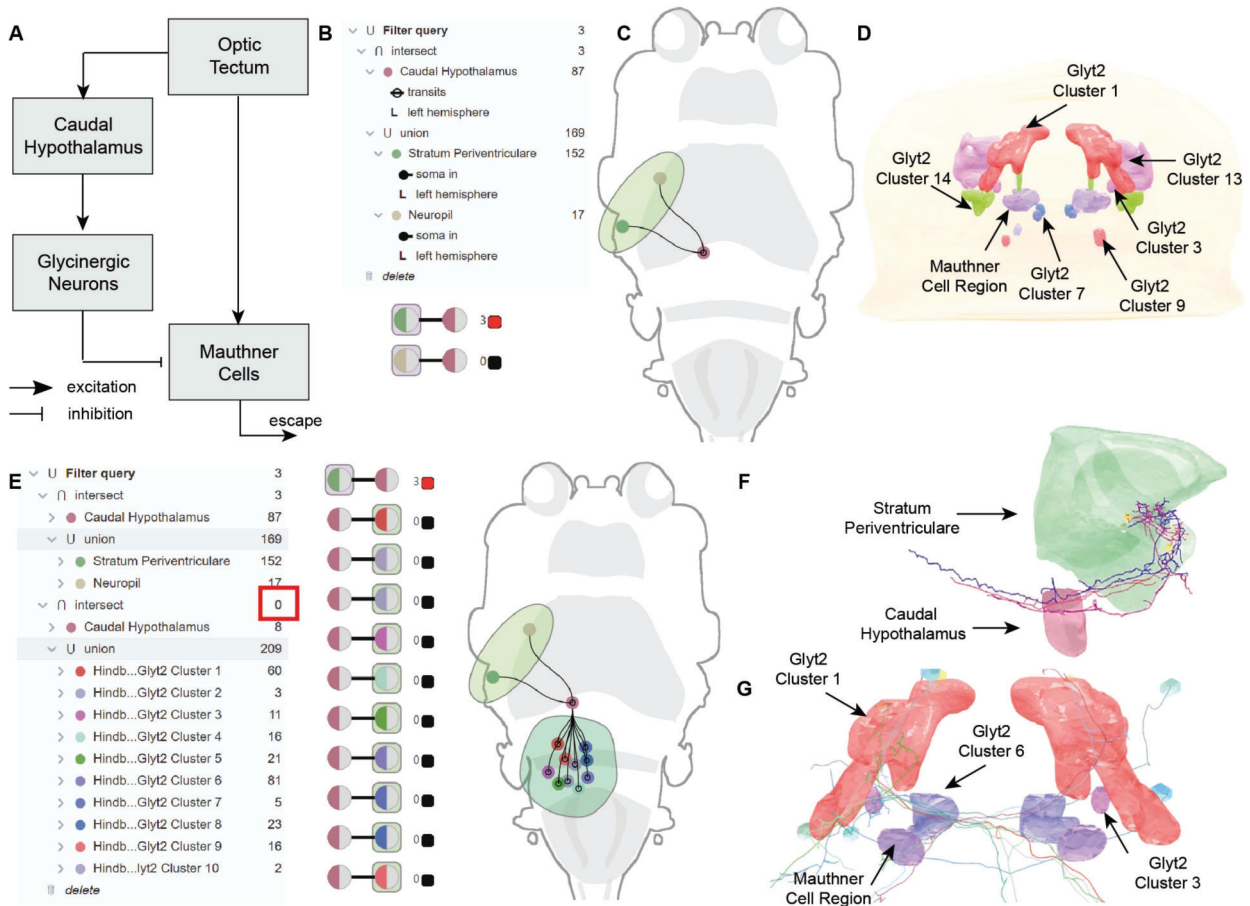
Fig. 8. Case study 1 . A : Graphical illustration of the circuit hypothesis regarding the inhibiting escape behavior, proposed by Yao et al. [50], described in more detail in case study 1 (Section VI-C). B : Query builder (Section V-A1); C : Circuit viewer (Section V-C1); D : 3D visualization of glycinergic interneuron clusters that are located next to the Mauthner cell region. E : Example of a query, described in Section VI-C. The number of neurons satisfying each subquery are displayed with a subquery returning no results (red box); F : 3D view revealing the connectivity of neurons that have their soma in the stratum periventriculare and pass through the caudal hypothalamus; G : 3D view revealing the connectivity of neurons transiting through glycinergic interneuron clusters and projecting to the Mauthner region.
