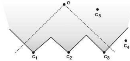
Fig. 3 Illustrating the sets W_e^C . c_1 , c_2 and c_3 are the choice events in e 's causal past indicated by the dashed lines ( c_4 and c_5 are outside that region). The region W_e^C is shaded grey; the boundary is not part of W_e^C . Note that W_e^C contains all events above c_5 , even though events in different continuations of c_5 are incompatible
