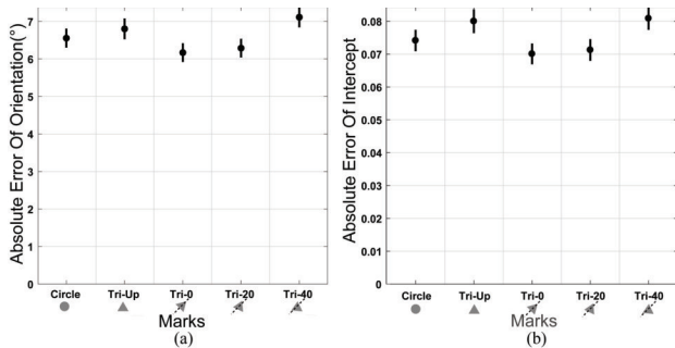
Figure 5: Results of Hypothesis 1 in Experiment 1: effect of mark orientation on the accuracy of estimating trend orientation (a) and trend intercept (b). Triangle marks with an orientation consistent with the actual trend result in the smallest error, while Tri-40 results in the largest errors.
