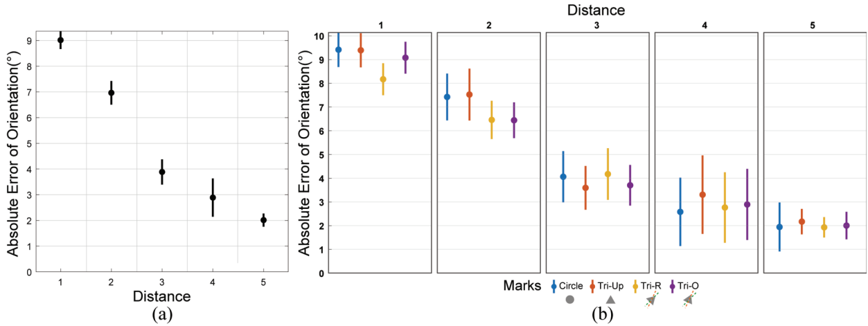
Figure 11: Results of Hypothesis 2 in Experiment 2: (a) Effect of outlier distance on the accuracy of trend orientation estimation; (b) interaction effect between outlier distance and mark orientation on the accuracy of trend orientation estimation.
