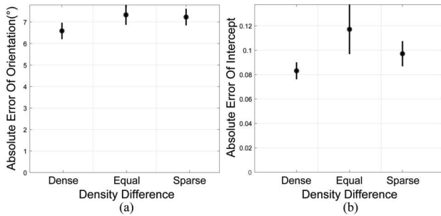
Figure 12: Results of Hypothesis 3 in Experiment 2: effect of outlier cluster density on estimating trend orientation (a) and intercept (b).
