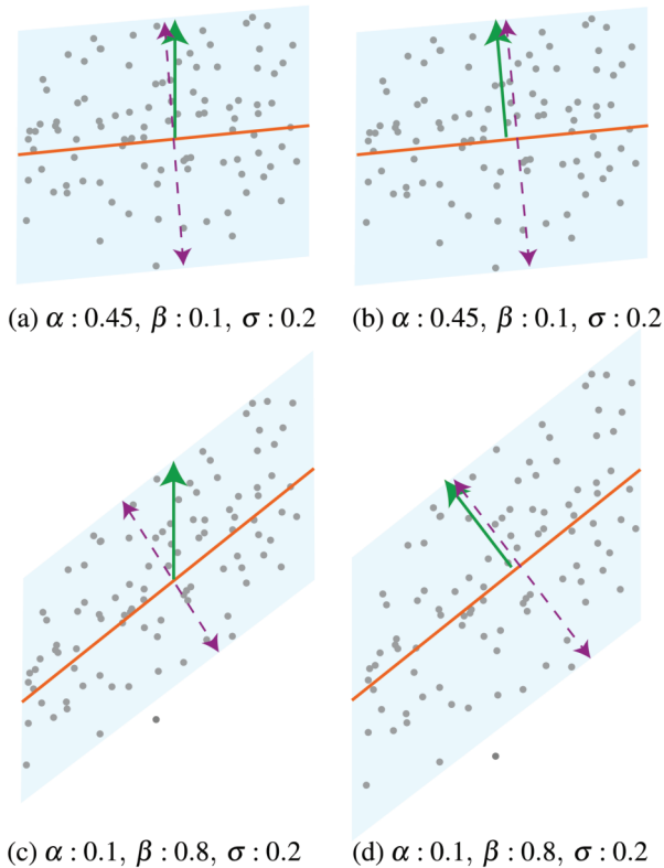
Figure 2: Comparison of point sets generated by adding Gaussian residuals along the vertical direction in green (a,c) and orthogonal direction in purple (b,d) to the trend line (shown in orange).
