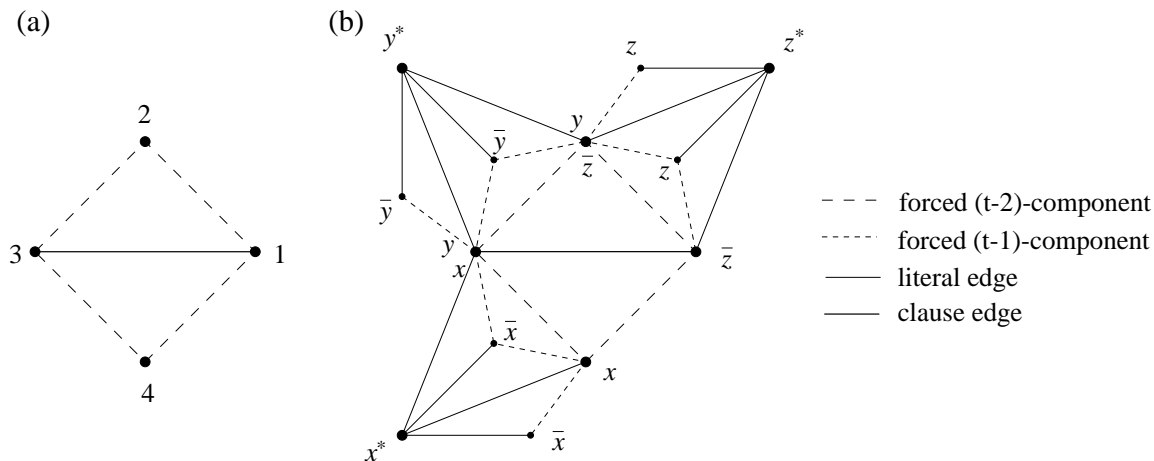
Figure 3: (a) Clause component, (b) the truth assignment testing component for clause c = x \vee y \vee \bar{z} using the symbolic representation for relevant blocks of the variable components
