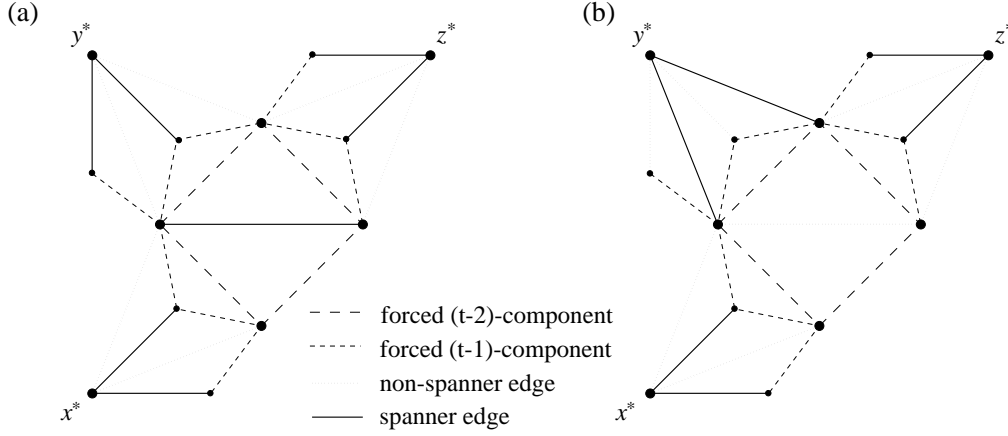
Figure 4: The minimum t -spanner in the truth assignment testing component
