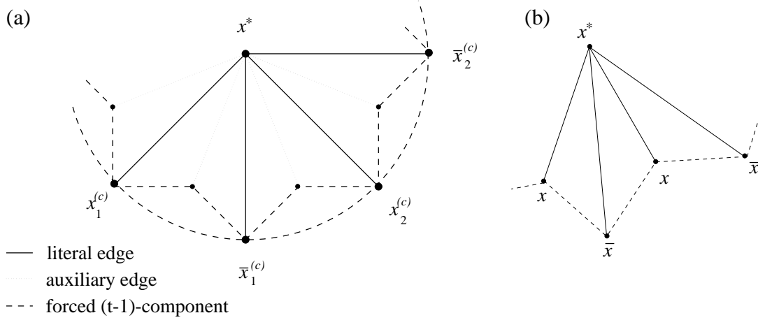
Figure 2: (a) Part of the variable component T_x for variable x occurring in clause c , (b) its symbolic representation
