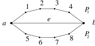
Figure 1: Forcing edge \{a, b\} into a 5-spanner
