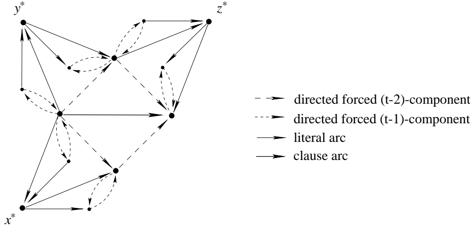
Figure 8: The directed truth assignment testing component for unweighted digraphs
