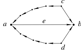
Figure 6: Forcing arc (a, b) into a 5-spanner
