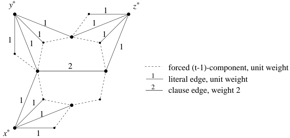
Figure 5: The truth assignment testing component in the weighted case
