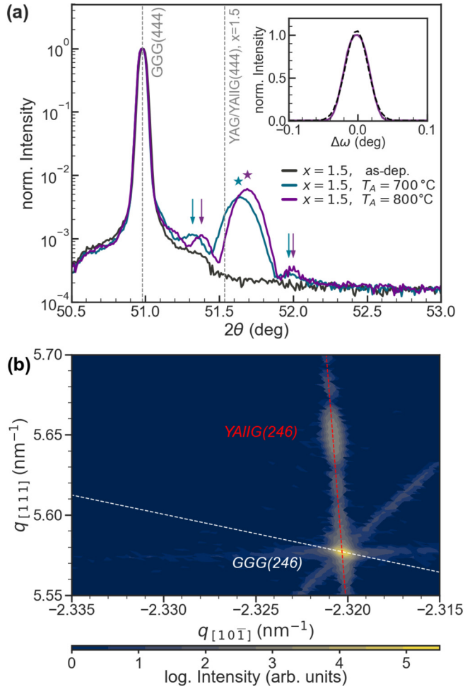
FIG. 2. XRD-analysis of GGG/YAlIG films with x = 1.5 : (a) Symmetric 2\theta - \omega scan of films annealed at different temperatures. The \star indicates the YAlIG (444) peak, the arrows indicate the first Laue oscillation of YAlIG. The inset shows the \omega scan of the YAlIG film annealed at 800^\circ\text{C} . The dashed line indicates the numerical fit of the data to a Pseudo-Voigt function. (b) RSM of the asymmetric (246) peak of a sample annealed at 800^\circ\text{C} , where the white dashed line indicates the peak position for a growth of fully relaxed YAlIG and the red dashed lines indicate the peak position for a growth of fully strained YAlIG.
