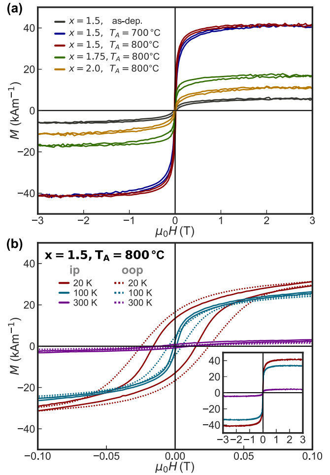
FIG. 6. SQUID-VSM M(H) hysteresis loops of YAlIG thin films grown on YAG. (a) In-plane M(H) hysteresis loops up to \mu_0 H = \pm 3 T at 20 K for different annealing temperatures and compositions. (b) In-plane M(H) hysteresis loops at different temperatures for fields up to \mu_0 H = \pm 0.1 T for a sample with x = 1.5 annealed at T_A = 800 °C. The inset shows the complete field range of \mu_0 H = \pm 3 T.
