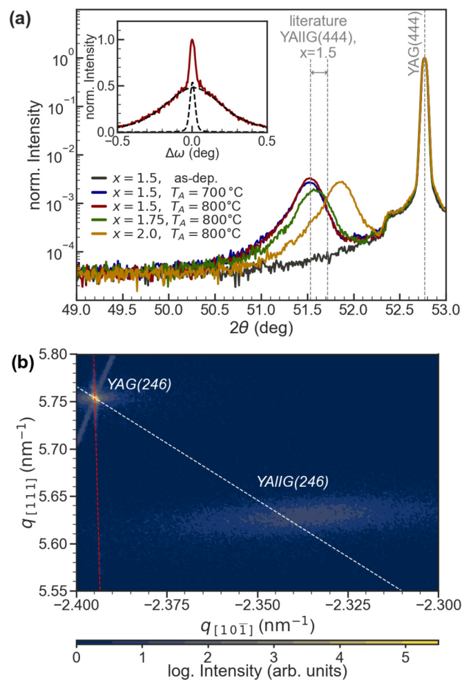
FIG. 1. XRD-analysis of YAG/YAlIG films: (a) Symmetric 2\theta - \omega scan for different annealing conditions and compositions. The two gray dashed lines denote the range of values reported in literature for x = 1.5 [25,30,39–42]. The inset shows the \omega scan of the YAlIG film annealed at 800^\circ\text{C} , x = 1.5 . The dashed lines indicate the numerical fit of the data to two independent Pseudo-Voigt functions. (b) RSM of the asymmetric (246)-peak of a sample annealed at 800^\circ\text{C} , x = 1.5 . The white dashed line indicates the peak position for a growth of fully relaxed YAlIG and the red dashed lines indicates the peak position for a growth of fully strained YAlIG.
