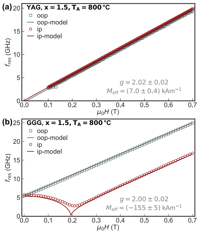
FIG. 7. FMR resonance f_{\text{res}} as a function of the applied magnetic field H at a temperature of 200 K for a YAIIG sample grown on YAG (a) and one sample grown on GGG (b). The modeled curve is based on the approach by Baselgia et al. [56] and the total free energy density described in Eq. (1). The corresponding M_{\text{eff}} and g are displayed in the plot.
