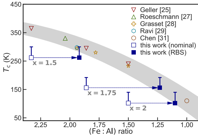
FIG. 5. Curie temperature T_c of YAlIG with different Fe:Al ratios, reported in the literature [25,27–29,31,39] and the results of this study. The shaded area is a guide for the eye for the expected range of T_c based on the literature. For the results of this study, the errorbars indicate the upper limit T_{c,max} and the arrow indicates the shift due to the difference between the nominal (\text{Fe} : \text{Al})_{\text{target}} ratio and the (\text{Fe} : \text{Al}) ratio measured via RBS.
