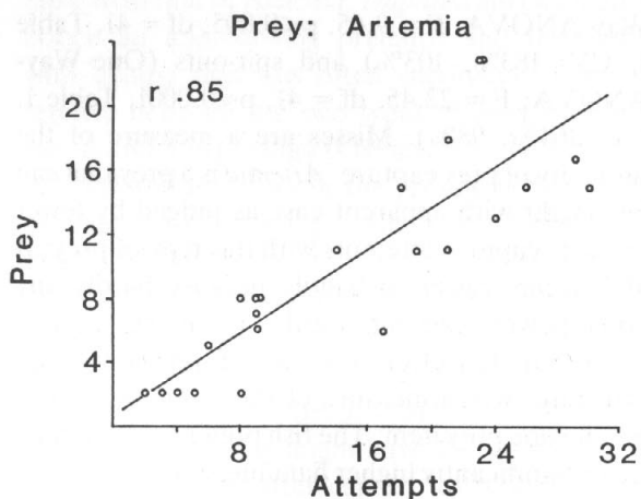
Fig. 3. X-Y-plot of attempts versus capture rate with Artemia as prey. The regression line has the formula: capture rate = 0.77 + 0.63 \times attempts. 72% of the variation in the variable capture rate is explained by the number of attempts made by the fish (regression analysis, F = 55.24 , df = 22 , p < 0.001 , r = 0.85 , p < 0.05 ). The slopes in Figure 3 and 4 are the capture efficiency.
