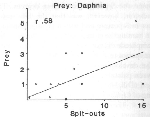
Fig. 5. X-Y-plot of spit-outs versus capture rate with Daphnia as prey. The regression is significant (regression analysis, F = 8.68 , df = 18 , r = 0.58 , p < 0.01 ). 34% of the variation in capture rate is explained by the variable 'spit-out'. The regression line has the formula: capture rate = 0.23 + 0.19 \times \text{spit-outs} .
