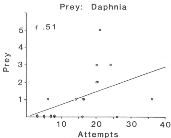
Fig. 4. X-Y-plot of attempts versus capture rate with Daphnia as prey. The regression line has the formula: capture rate = -0.095 + 0.079 \times attempts. The regression is significant (regression analysis, F = 5.93 , df = 18 , r = 0.51 , p < 0.05 ). 26% of the variation in capture rate is explained by the variable 'attempts'.
