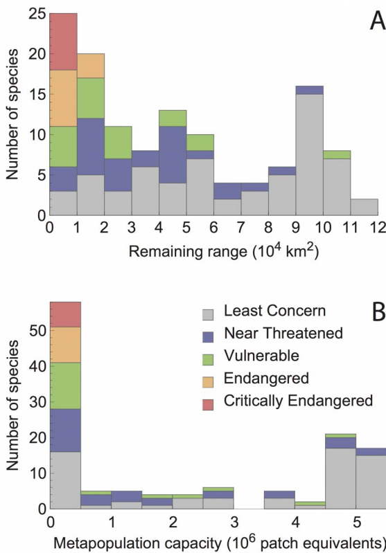
Figure 2. For 127 passerine birds of the Atlantic forest of Brazil, differences are evident between two measures of extinction risk: A) the area of a bird’s remaining range; B) metapopulation capacity, which accounts for range fragmentation as well as area. Colors indicate IUCN Red List categories with red, orange, and green being the three ‘threatened’ categories. When accounting for the long-term extinction risk associated with fragmentation, a distinct group of 57 species with very low metapopulation capacity becomes apparent, of which 28 are deemed non-threatened by BirdLife. doi:10.1371/journal.pone.0065357.g002
