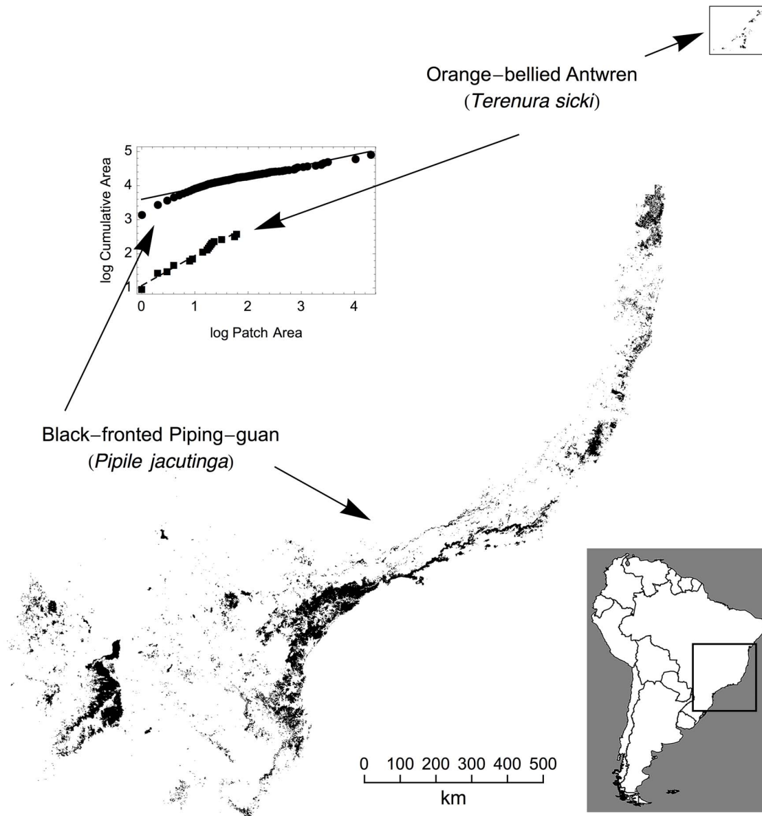
Figure 1. Cumulative area plots of two Atlantic forest birds, the large-ranged black-fronted piping-guan ( Pipile jacutinga ) and the small-ranged orange-bellied antwren ( Terenura sicki — highlighted with a box). Graph axes are the logarithm of cumulative area in patches up to a given size, versus the logarithm of that patch size. The lines are fitted linear regressions. A steep (more positive) slope, e.g. orange-bellied antwren, indicates that a range is composed mainly of relatively larger patches. Shallow slopes, e.g. black-fronted piping-guan, indicate birds with ranges composed of relatively many smaller forest fragments. Counter-intuitively, while the guan has a larger overall range and larger patches within that range, the shallower slope of its plot suggests that it is more fragmented (see text for further discussion). doi:10.1371/journal.pone.0065357.g001
