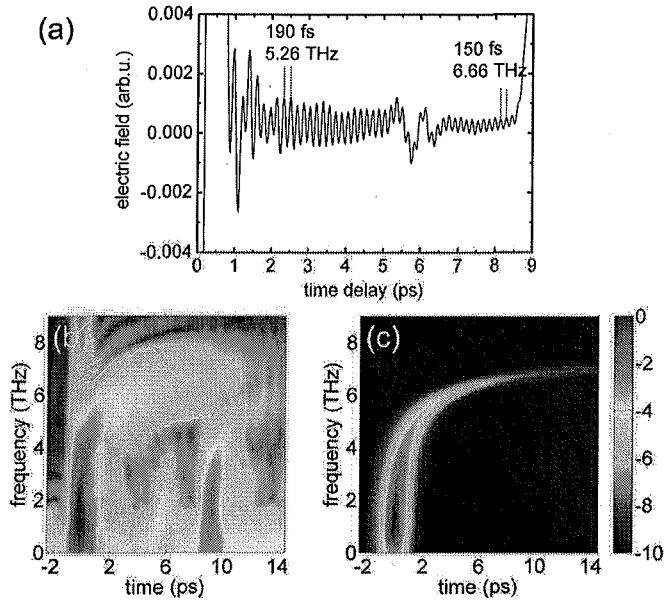
Fig. 2. (a) Zoom-in into the first picoseconds after the main THz pulse. The larger delay of higher frequency components is readily visible in the time-domain. (b) FFT with a sweeping time window of 1 ps length of the time-domain data shown in (a). (c) Corresponding calculated 2D plot of the delayed frequency components, generated from the phonon-polariton dispersion relation. The color of both 2D plots maps the FFT intensity onto a logarithmic scale.
