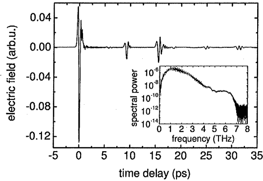
Fig. 1. Transient with multiple reflections of the THz pulse in the THz emitter substrate and GaP detection crystal. The inset shows the corresponding Fourier transform.
