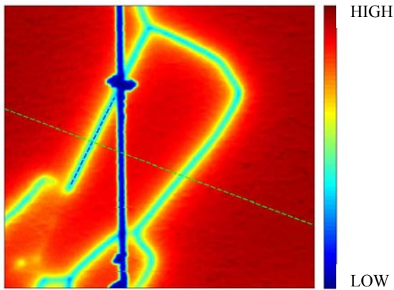
Figure 2: LBIC map of short circuit current @ 833 nm for a two GB situation
