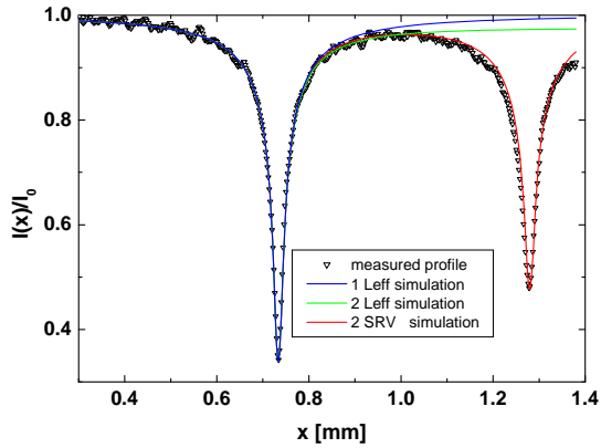
Figure 5: comparison between ‘one L_{eff} ’, ‘two L_{eff} ’ and ‘two SRV’ model at the cutline defined in Fig. 4
