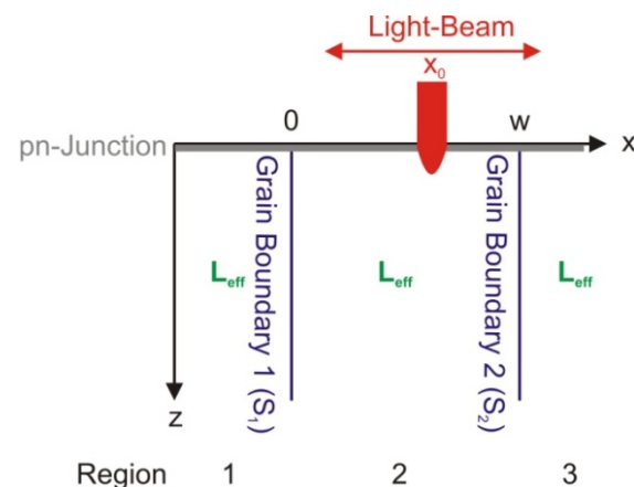
Figure 1: Schematic of the diffusion problem. Requirements and justifications of the model can be found in [2].
