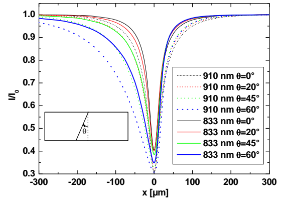
Figure 6 : Simulation of a grain boundary contrast profile when the GB is tilted by an angle \theta with an infinite SRV, L_{eff}=100 \mu\text{m} on a 250 \mu\text{m} thick structure for 910 and 833 nm laser wavelength
