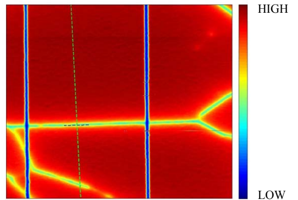
Figure 4: LBIC map of short circuit current @ 833 nm for another two GB situation
