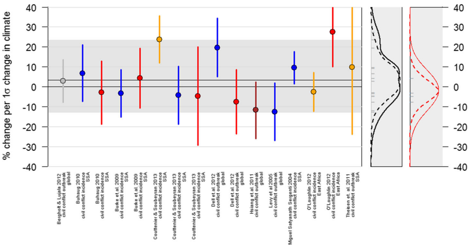
Fig. 1 Modern empirical estimates for the effect of climate variability on civil conflict. The markers illustrate the estimated percentage change in conflict with a 1\sigma increase in temperature (red), loss of rainfall (blue), or increase in drought (orange), El Niño-like conditions (brown) or increase in severity of climatic natural disasters (gray). Whiskers denote the 95 % confidence interval. The solid horizontal line indicates the median climate effect with the 95 % highest density interval in grey, based on a Bayesian hierarchical model. The panels at the right show the distribution of results from all candidate studies (black) or those focusing squarely on temperature effects (red); solid lines represent the variance-weighted distribution while dashed lines depict the Bayesian hierarchical distribution. Studies listed alphabetically
