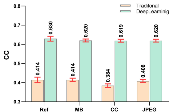
FIGURE 9. Average performance (measured by the CC metric) of traditional versus deep learning-based saliency models on different distortion types on the CUDAS database. Ref, MB, CC and JPEG represent reference, motion blur (MB), contrast change (CC), and JPEG compression (JPEG), respectively. The error bars indicate a 95% confidence interval.
