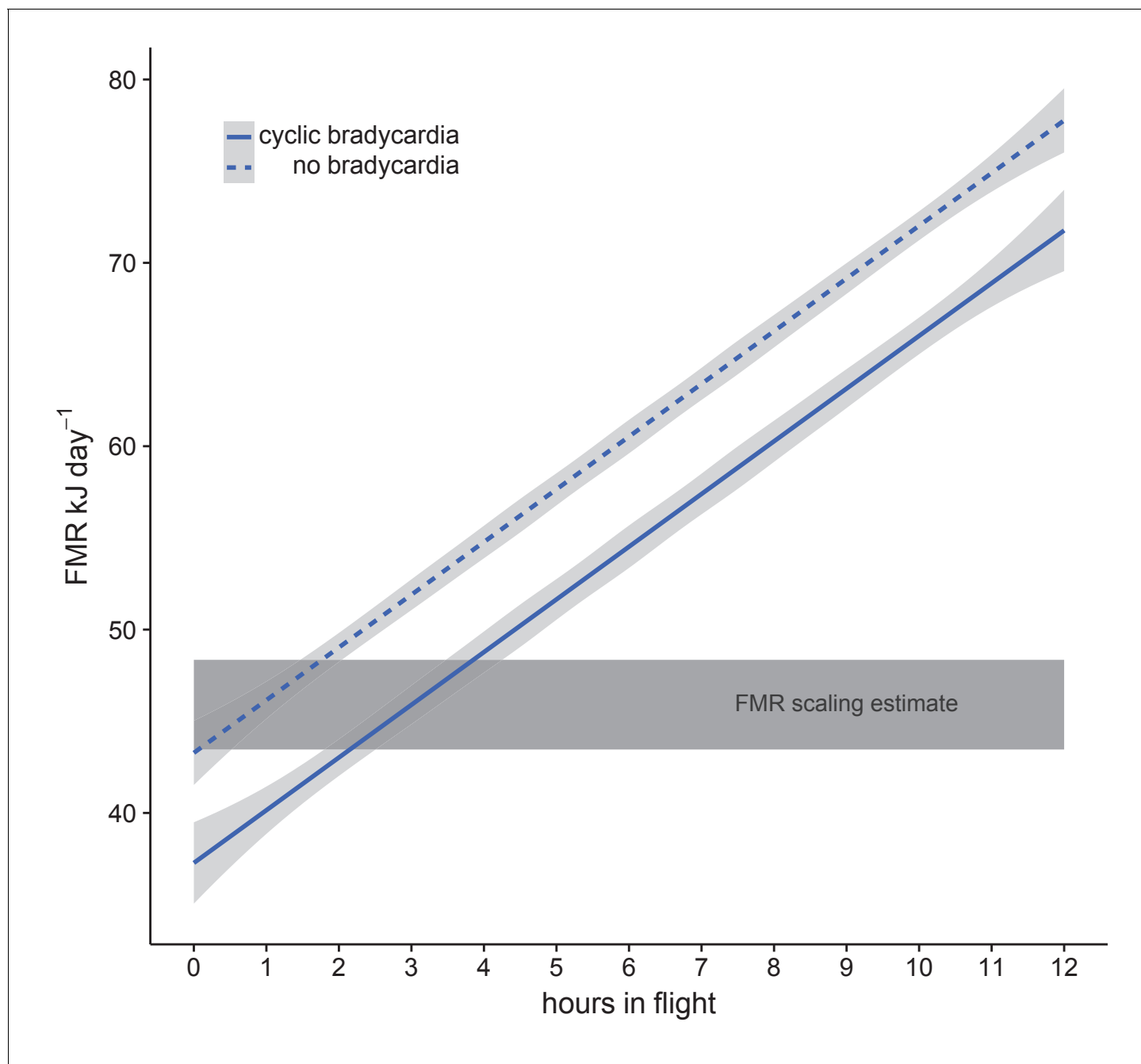
Figure 3. Mean field metabolic rate \pm 95\% CI estimated by the number of hours spent in flight with (solid line) and without (dashed line) daily cyclic bradycardia. A conservative estimate of two hours flight and a mean FMR of 45.79 \text{ kJ day}^{-1} is based on our radio tracking observations of free-flying bats in their natural environment. This is within the estimates from the Speakman (2005) scaling relationship (grey box) for the range of body masses (16–19 g) measured in this population.
