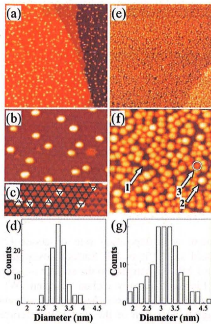
FIG. 2. (Color online) STM topographs obtained after deposition of 0.25 ML Ni at 150 K (a), (b), (c), and 1.50 ML Ni (e), (f). The corresponding histograms of clusters diameter vs the number of clusters are displayed in [(d) and (g)]. The Moiré superstructure in (c) is outlined by a grid. Numbers in (f) refer to different kinds of NCs. Image sizes are (a) and (e) 200 \times 200 \text{ nm}^2 ; (b) 50 \times 35 \text{ nm}^2 ; (c) 50 \times 15 \text{ nm}^2 ; and (f) 50 \times 50 \text{ nm}^2 . Tunneling parameters: (a) +2 V, 0.14 nA; (b) +1.02 V, 0.13 nA; (c) +0.95 V, 1.56 nA; (e) +1.12 V, 2 nA; and (f) +1.29 V, 0.8 nA.
