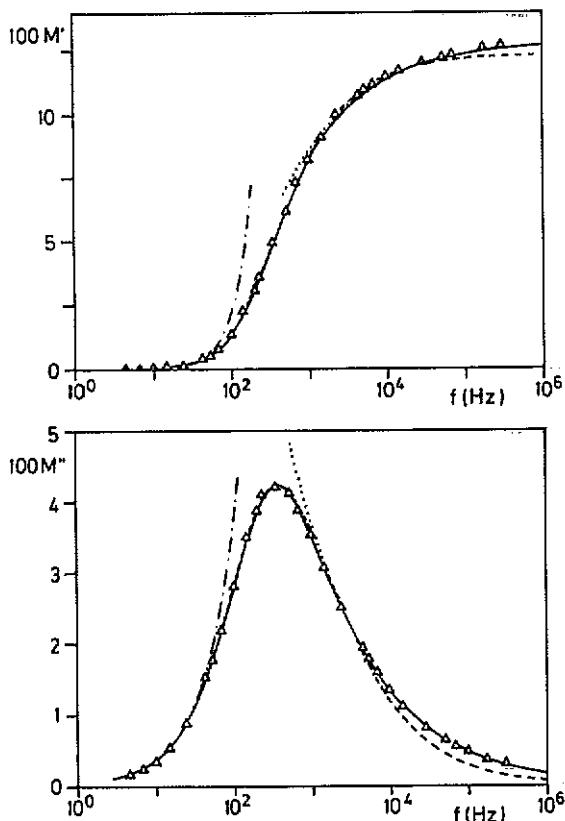
Figure 1. Reactive part M' and absorptive part M'' of the CKN dielectric modulus at 71.4°C (triangles) together with a Kohlrausch fit with exponent \beta = 0.64 (broken curves) from Howell et al (1974). The dotted curves are von Schweidler asymptotes (2) for exponent b = 0.44 . The chain curves are fits to the stochastic behaviour M' \propto \omega^2 , M'' \propto \omega . The full curves are MCT results for the model (40) and (41), specified in the text.
