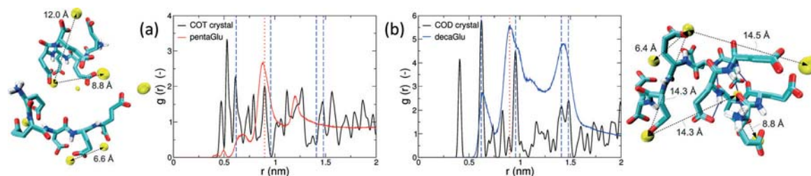
Fig. 3 Pair correlation functions of \text{Ca}^{2+} ions during the H-REMD simulations of 5Glu (a) and 10Glu (b) in comparison to those in calcium oxalate trihydrate (a) and dihydrate (b), with exemplary snapshots from the H-REMD simulation that feature characteristic calcium distances. Vertical lines denote significant \text{Ca}^{2+} - \text{Ca}^{2+} distances in the two \text{CaC}_2\text{O}_4 pseudopolymorphs (blue dashed lines: COD crystal; red dotted line: COT crystal).
