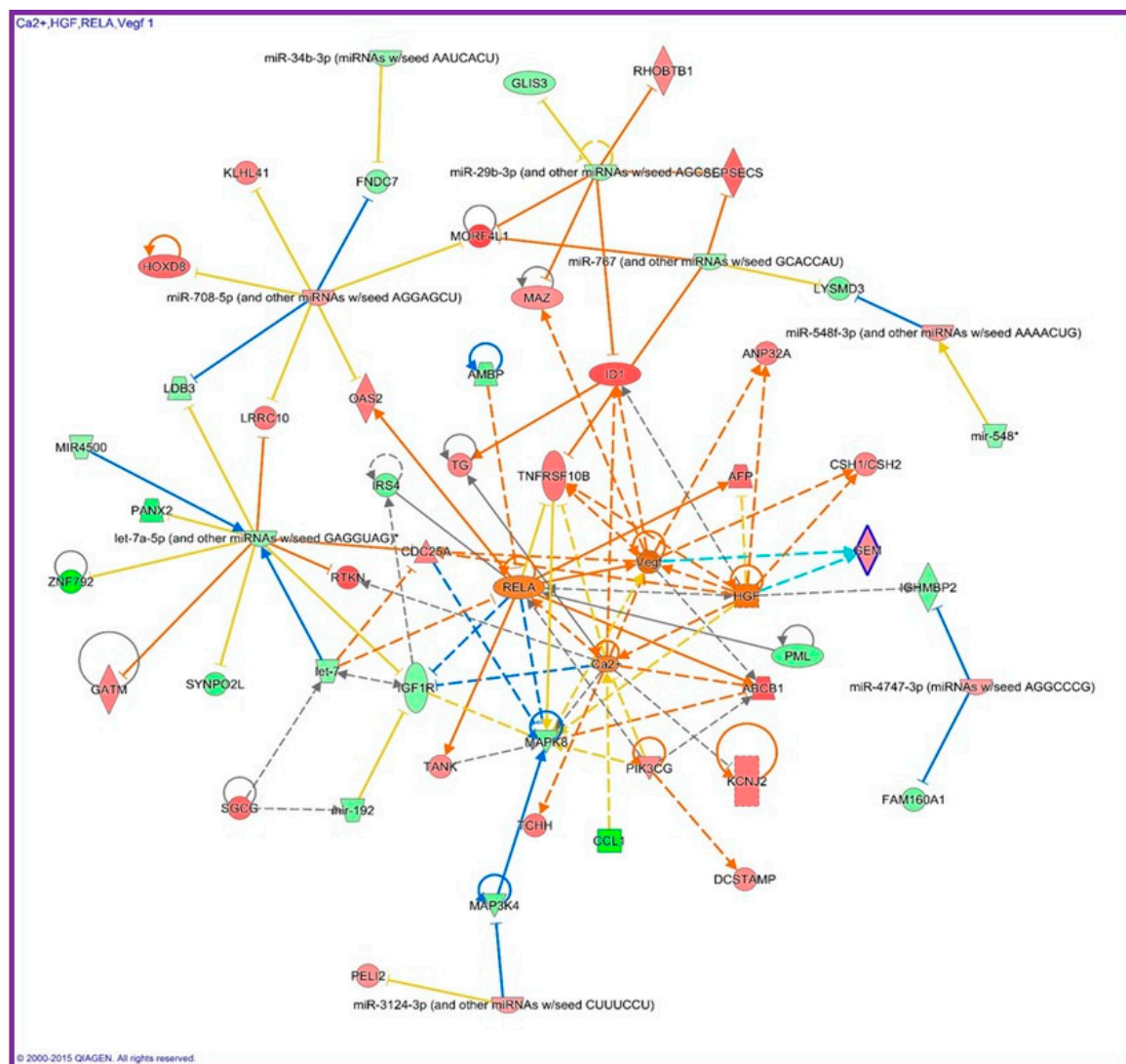
Figure 1. Interaction network identified with genes and miRNAs that were differentially expressed in human fibroblasts after flown on the international space station for 3 days. The chart was generated using Ingenuity Pathway Analysis (Qiagen, Germantown, MD, USA). Activation of NF- \kappa B in space may be responsible for the faster cell proliferation by upregulating HGF and VEGF [30].
