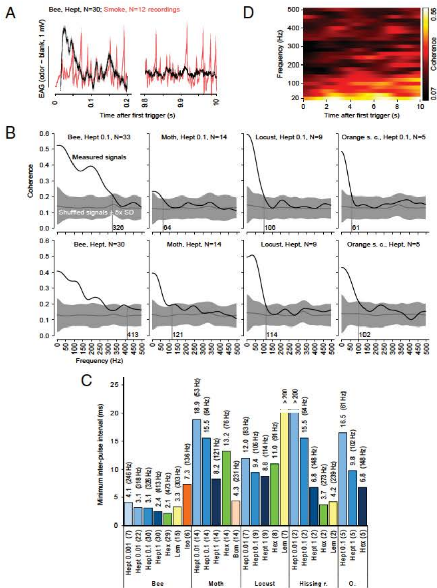
Fig. 4. Antennal responses track odor fluctuations in the hundreds of Hertz range during a persistent broadband stimulus. (A) TiCl 4 smoke signals (red, n = 12 ) and odor evoked EAG responses (black, 20 Hz high pass filtered, onset truncated, n = 30 ) (mean \pm SEM) during 0–0.2 and 9.8–10 s of a 10 s long broadband frequency stimulus train with random pulse durations and intervals. (B) Coherence between mean EAG responses and TiCl 4 smoke signals (black) and coherence between mean EAG response and a shuffled TiCl 4 smoke signal (gray, mean \pm 5 SD). The first 1,000 and the last 100 ms of the 10 s long broadband stimulus were skipped to avoid onset/offset effects. Coherence was defined significant when it was larger than the coherence for the shuffled data plus 5 SD. Values at the vertical lines are the maximum frequencies at which the EAG response shows significant coherence. (C) Temporal resolution of EAG responses quantified as the minimum inter-pulse interval in milliseconds ( 1/\text{maximum pulse frequency} ) at which the coherence was significant, i.e., larger than the coherence for the shuffled data plus 5 SD. The corresponding pulse tracking frequencies are given in parentheses. Experiments are grouped at the bottom by species and then odorant and dilution, with the number of antennae in parentheses. (D) Time resolved, color coded coherence between the mean honey bee EAG response to undiluted 2 heptanone and the mean TiCl 4 smoke signal (same data as in Fig. 4A). The time resolved coherence indicates the degree to which the EAG response is phase locked to the fluctuations of the odor concentration, as opposed to merely matching the frequency. Substantial coherence at high frequencies is visible throughout the odor presentation, indicating that tracking can persist for several seconds.
