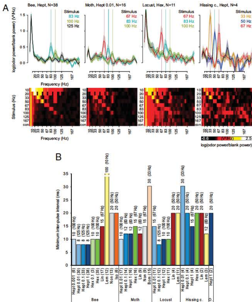
Fig. 3. Antennal responses track pulses at 125 Hz in a 1 s long odor stimulus. (A) Periodograms (mean \pm SEM) of the EAG responses for the three highest resolved pulse frequencies for different odors in different insect species, and color coded periodograms for all pulse series for the same species odor combination. A peak in the periodogram indicates that the EAG response followed that stimulus frequency. (B) Temporal resolution of EAG responses quantified as the minimum inter-pulse interval in milliseconds ( 1/\text{maximum pulse frequency} ) that an EAG response could follow. Minimum inter-pulse intervals were determined by locating the peak of the average periodogram in a \pm 20 Hz window around the stimulus frequency. Pulse following was ascertained if the negative SE of the peak location rose above the positive SE of the trough location within that window. The corresponding pulse tracking frequencies are given in parentheses. The number of antennae is given in parentheses above the odorant.
