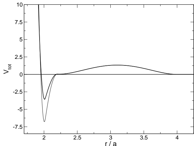
FIG. 1: Interaction potential for two particles with the average radius. The polymer fractions are \phi_p = 0.42 and \phi_p = 0.25 for the thin and thick curves, respectively (values close to the glass transition in the simulation and MCT, respectively). Note that in our units, the thermal energy is k_B T = 4/3 .
