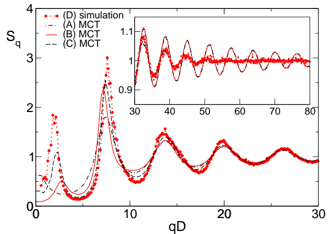
FIG. 3: Critical S_q at the boundaries of the gel phase: Black dashed-dotted, red full and black dashed lines mark results from (A), (B) and (C). The red diamonds indicate S_q at \phi_p = 0.42 , which is close to the arrested state in the simulation (D). In the simulation, the prepeak at qD \approx 2.5 rises and shifts to smaller q -values with increasing polymer concentration. The inset gives an enlarged view of the q -tail where systems (A,B) show pronounced oscillations driven by the short-ranged attraction.
