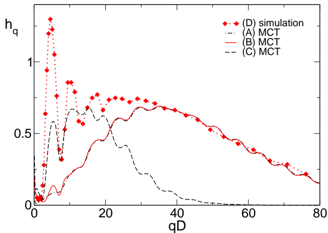
FIG. 6: Critical amplitudes in simulation (D) (red diamonds) and MCT (A,B,C) (black dashed-dotted, red full, black dashed) close to dynamic arrest. Because of the different \alpha -times in simulation and theory the MCT-results for (A,B) were scaled on the simulation results.
