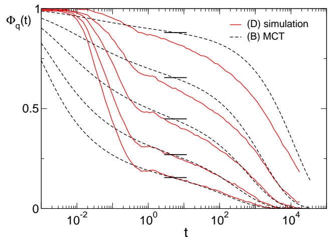
FIG. 8: Density correlation functions in simulation ((D) red solid lines) and MCT calculations in model (B) (black dashed lines): The horizontal black bars indicate the critical plateau values of f_q^c in MCT. The wavevectors from bottom to top are qD = 57.1, 45.9, 33.9, 22.7, 12.5 . The short time diffusion coefficient was set to D^s/D^2 = 0.133 . The theoretical curves correspond to a polymer concentration of \phi_p = 0.2461 , which means a separation parameter of about \epsilon_{MCT} = -0.001 . The simulation results were obtained for a polymer concentration \phi_p = 0.42 , which corresponds to a separation parameter of \epsilon_{simu} = -0.015 .
