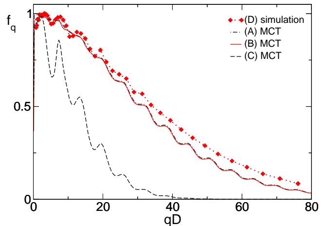
FIG. 4: Critical nonergodicity parameters f_q^c at the transition in the simulation (D) (red diamonds), from MCT with monodisperse (A,B) S_q (black dashed-dotted and red full line) and polydisperse (C) S_q (black dashed line). Serious differences occur, when the average S_q of a polydisperse system is used as input to a monodisperse theory; the shape of f_q^c for (C) resembles more the one of a repulsive glass.
