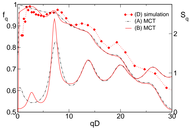
FIG. 5: Enlarged view of the nonergodicity parameters of Fig. 4 and structure factors in the low- q -region: Minor differences in f_q^c show up in the region qD \leq 10 only, where also the input S_q differs considerably. Simulation data ((D) red symbols) agree qualitatively with the model calculation (B) including the barrier.
