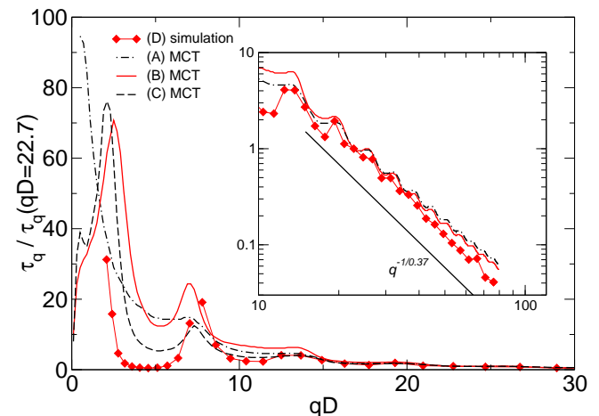
FIG. 7: \alpha -relaxation times \tau_q in MCT for the systems (A),(B),(C) (black dashed-dotted, red full, black dashed line) and in the polydisperse simulation ((D) red diamonds). The curves are normalized to the value of \tau_q at qD = 22.7 . In the inset, the results for models (A) and (B) and simulation (D) are shown in a log-log plot. The straight line gives the asymptotic behavior \tau_q = q^{-1/b} valid for large q with the corresponding von Schweidler b = 0.37 obtained previously.
