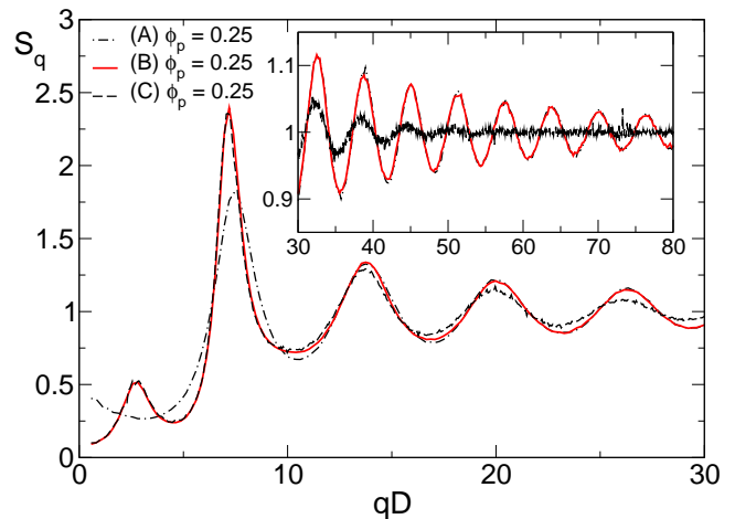
FIG. 2: S_q from MD-simulations at a colloid packing fraction of \phi_c = 0.40 and a polymer concentration of \phi_p = 0.25 , which is in the gel close to the critical point in MCT. The repulsive barrier affects S_q in the region below qD \leq 13 ; system (A) without barrier (dashed-dotted, black) shows neither a prepeak nor a primary peak which is as high as in systems (B,C) with barrier (full red, dashed black). The inset demonstrates that polydispersity causes the q -tail oscillations in S_q to be suppressed for large wavevectors. The S_q for the polydisperse model (C) falls below the noise level for qD \geq 45 , whereas the monodisperse systems (A) and (B) virtually coincide there.
