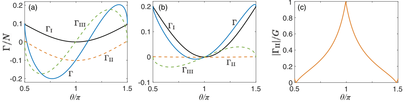
Figure 4. Normally-ordered second moment \Gamma of the electro-optic signal calculated according to Equations (7), (9), and (11) for different phase shifts \theta . a) \Gamma according to the level scheme shown in Figure 1b. The blue line depicts \Gamma for the full quantum treatment given by Equation (6). It is given by the sum of the classical contribution \Gamma_I [black line, cf. Equation (7)], the contribution stemming from the quantum susceptibilities \Gamma_{II} [dashed orange line, cf. Equation (9)] and the cascading contribution \Gamma_{III} [dashed green line, cf. Equation (11)]. b) Off-resonant case with \omega, \Omega \ll \omega'_{g'g}, \omega'_{fg} . The length L of the nonlinear medium with respect to the strength of the nonlinear susceptibilities is chosen such that the maximal value of \Gamma can still be regarded as a small correction to the shot noise. In this case, a maximum contribution of 0.2N was adopted. c) Ratio of the absolute strength of the quantum contribution |\Gamma_{II}| to the combined absolute strengths of each contribution G = |\Gamma_I| + |\Gamma_{II}| + |\Gamma_{III}| for the level scheme shown in Figure 1b. The normally-ordered second moment \Gamma is almost entirely determined by the quantum contribution \Gamma_{II} for the half-wave plate configuration, given by \theta = \pi .
