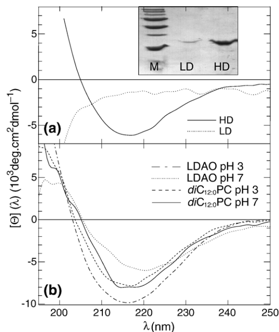
Figure 4. (a) Folding of hVDAC1 into lipid bilayers is near quantitative. Sucrose density gradient centrifugation of folded hVDAC1 in diC 12:0 PC resulted in two layers of lower (LD) and higher density (HD). The HD layer contained more than 92% of hVDAC1. The CD spectra indicated hVDAC1 was folded in the HD (—), but not in the LD (· · ·) layer. Inset: SDS-PAGE analysis of both layers, with molecular weight markers (M). (b) The CD spectra of hVDAC1 in LDAO micelles at pH 3 (— · —) and immediately after adjustment of the pH to 7 (· · ·) indicated a strong conformational change upon pH adjustment, while hVDAC1 spectra in diC 12:0 PC bilayers were very similar at pH 3 (— · —) and at pH 7 (—).
