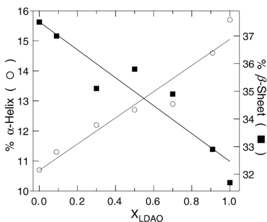
Figure 7. The contents of \alpha -helix (○) and \beta -sheet (■) in hVDAC1, derived from CD spectra (Figure 6 and Table 3), are a function of the molar fraction of LDAO in binary mixtures with di C 12:0 PC. The molar amphiphile (LDAO+ di C 12:0 PC)/hVDAC1 ratio was 800.
