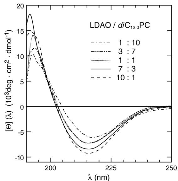
Figure 6. Normalized CD spectra of hVDAC1 in detergent/lipid mixed micelles of LDAO and diC_{12:0}PC . The increase in the spectral amplitude and the shift in the maximum of the spectra from \lambda \approx 195 nm to \lambda \approx 192 nm is characteristic for an increase in the \alpha -helical fraction at higher LDAO content in LDAO/ diC_{12:0}PC mixtures.
