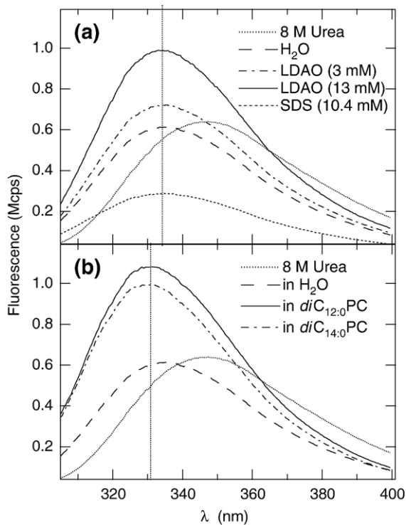
Figure 5. Fluorescence spectroscopy indicates a different microenvironment of the tryptophan residues of hVDAC1 in LDAO micelles and in lipid bilayers. (a) The fluorescence spectra of 1.3 \mu\text{M} hVDAC1 in 3 mM LDAO (---), in 13 mM LDAO (—), and in 10.4 mM SDS (---) have maxima at 335 nm. (b) The fluorescence spectra of hVDAC1 in an 800-fold molar excess of diC_{12:0}PC (—) or diC_{14:0}PC (---) have maxima at 330 nm. Also shown are fluorescence spectra of unfolded hVDAC1 in 8 M urea (···) and of aqueous hVDAC1 after urea dilution (—).
