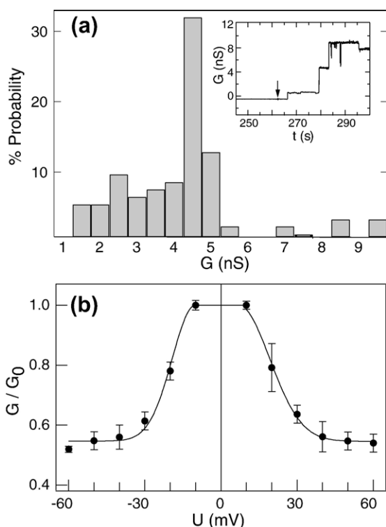
Figure 3. Single channel recordings demonstrate function of folded hVDAC1. (a) The histogram of hVDAC1 conductance indicates an average single channel conductance of G_0=4.5 nS at 10 mV for hVDAC1 in 1 M KCl. 94 single channel events were recorded at RT. The inset shows the stepwise increase in conductance across black lipid films of diPhPC at pH 7, upon addition (marked by ↓) of hVDAC1 solubilized in LDAO. (b) The conductance, G , of hVDAC1 is voltage-dependent. Above 10 mV, hVDAC1 forms channels of smaller conductance. Relative conductance, G/G_0 , is plotted as a function of the applied voltage.
