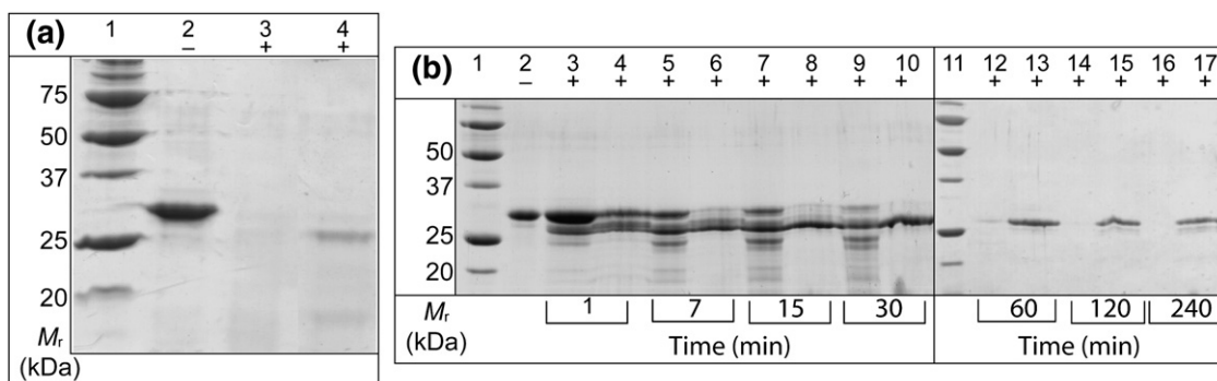
Figure 2. Pepsinolysis at pH 3 and analysis by SDS-PAGE demonstrates that hVDAC1 inserts into micelles or lipid bilayers. Protein standards are shown in lanes 1 and 11. (a) Unfolded hVDAC1 in urea migrates at 30 kDa (lane 2). Aqueous hVDAC1 is completely cleaved by pepsin (indicated by +) within 30 min (lane 3). After folding of hVDAC1 into diC 14:0 PC, pepsinolysis is incomplete and leads to a fragment with a size of \sim 26 – 27 kDa (lane 4) after 240 min. (b) Pepsinolysis of hVDAC1 in LDAO (lanes 3, 5, 7, 9, 12, 14, 16), and in diC 12:0 PC (lanes 4, 6, 8, 10, 13, 15, 17), indicate formation of a single fragment of \sim 26 to 27 kDa size in diC 12:0 PC bilayers that is present after 240 min of proteolysis. In LDAO, hVDAC1 is first cleaved into two major fragments of \sim 26 to 27 kDa and of \sim 24 kDa. Additional fragments of weaker intensity were also observed. Pepsinolysis of hVDAC1 in LDAO is complete after 60 min.
