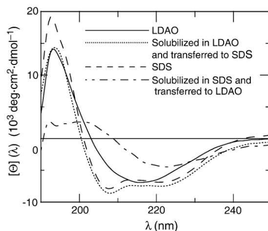
Figure 8. CD spectra of hVDAC1 in SDS indicated denatured hVDAC1 with high content of \alpha -helix secondary structure (—). CD spectra of hVDAC1 first incubated in LDAO (—) and then reconstituted into SDS (···) were similar to CD spectra obtained by direct reaction with SDS. SDS bound tightly to hVDAC1 and could not be replaced by LDAO and dialysis (- · - ·).
