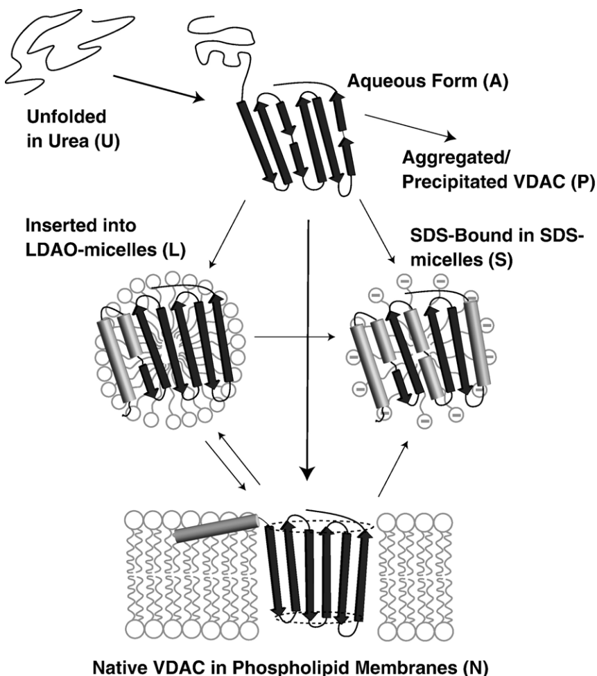
Figure 9. A tentative scheme for folding and insertion of hVDAC1 into lipid bilayers. From an unfolded form in urea (U) that does not display helix or sheet content, after urea dilution, hVDAC1 develops \sim 39\% \beta -strand structure (110 residues) in an aqueous intermediate (A). From this intermediate, hVDAC1 folds and inserts directly into lipid bilayers to its native form (N), composed of \sim 11\% \alpha -helix ( \sim 30 residues), \sim 36\% \beta -strand, and 23\% \beta -turn structure. Upon incubation with LDAO, hVDAC1 develops \sim 16\% \alpha -helix (45 residues), \sim 33\% \beta -strand ( \sim 93 residues), and 23\% \beta -turn structure. Upon reconstitution into phospholipid bilayers this secondary structure is converted to the secondary structure observed for direct refolding of denatured hVDAC1 into phospholipid bilayers. In SDS-micelles, SDS binds tightly to hVDAC1 and leads to formation of \sim 29\% \alpha -helical structure ( \sim 82 residues). The number of strands in these forms is not known.
