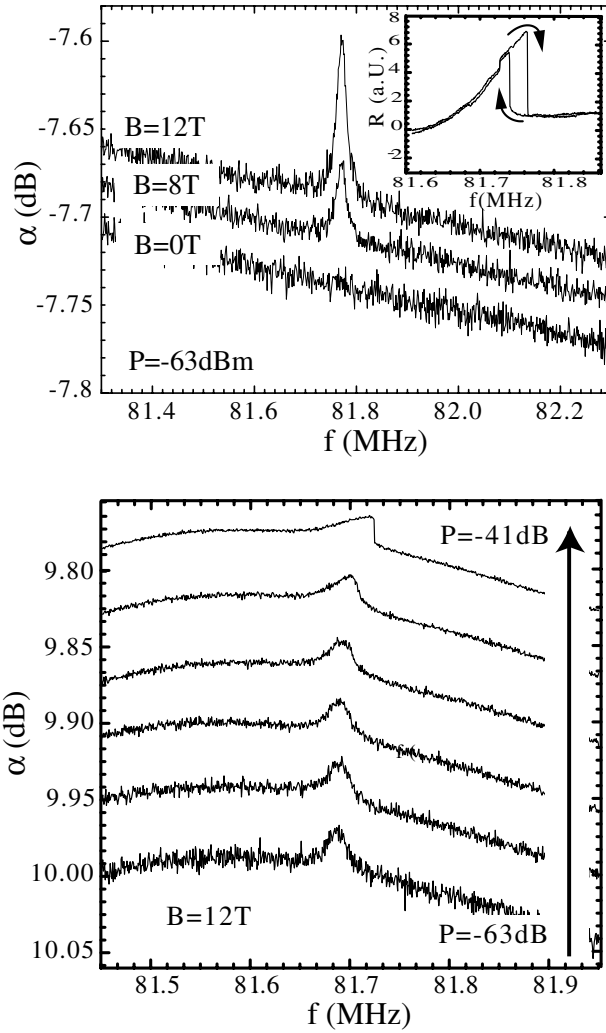
Figure 29. Top: measured resonances of a nanobeam: this mechanical resonator is 4.8 \mu\text{m} long, 170 \text{ nm} wide and 190 \text{ nm} thick, covered by a 50 \text{ nm} thick conducting Au layer. The magnetic field is oriented in the plane of the sample surface and perpendicular to the beam. The inset shows the observed hysteresis which emerges when tracing the frequency from low to high and the reverse. Bottom: resonances in the spectrum of a nanomechanical resonator detected by capacitive coupling.
