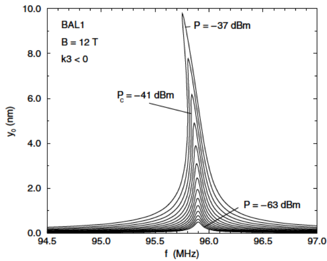
Figure 1. Nonlinear resonance trace for increasing values of F in equation (25), indicated by the power level P .
