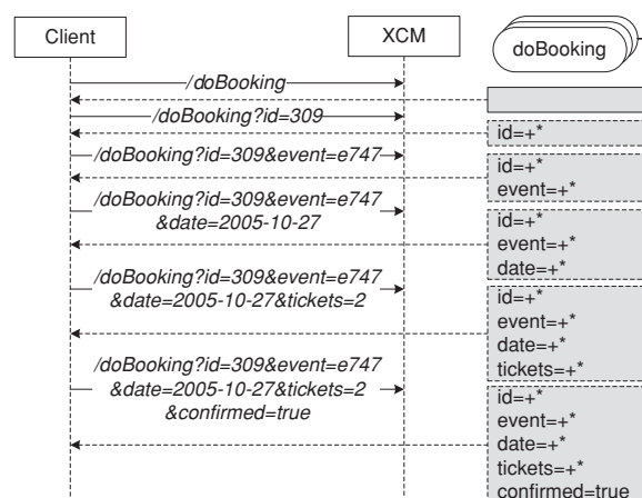
Fig. 6 Using variants to implement a booking process
