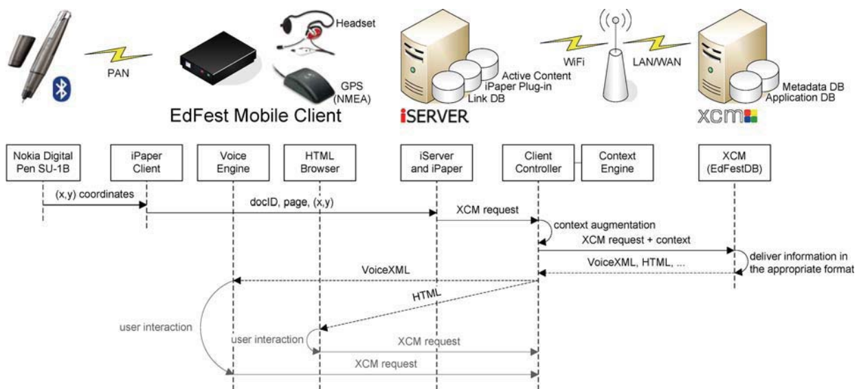
Fig. 5 EdFest architecture
