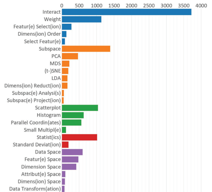
Fig. 3. The top 25 concepts we extracted from the 197 automatically selected papers (see Section III-C). Five colors contextualize each concept: ● Interaction, ● Dimensionality reduction (DR), ● Visualization, ● Statistics, ● Analysis space.
