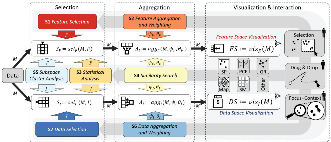
Fig. 5. In our framework for dual analysis, the dataset \mathcal{D} , is interpreted as a matrix. The matrix can then be transformed by a selection step, where the data can be reduced. Second, the result of this step is used for an aggregation step, which can be used to create representatives. Third and lastly, feature and data space are visualized using distinct but linked visualizations. All three steps take the result of the previous step as input. Scenarios are linked with the different steps of the pipeline by supplying parameterizations to the given operation sel_I (7), agg_I (8), vis_I (9), for data space operations, and sel_F (1), agg_F (2), vis_F (3). Analyst can interact with the visualizations, affecting the previous step and allowing for an immediate response, typical for dual analysis approaches, as described in Section V-D.
