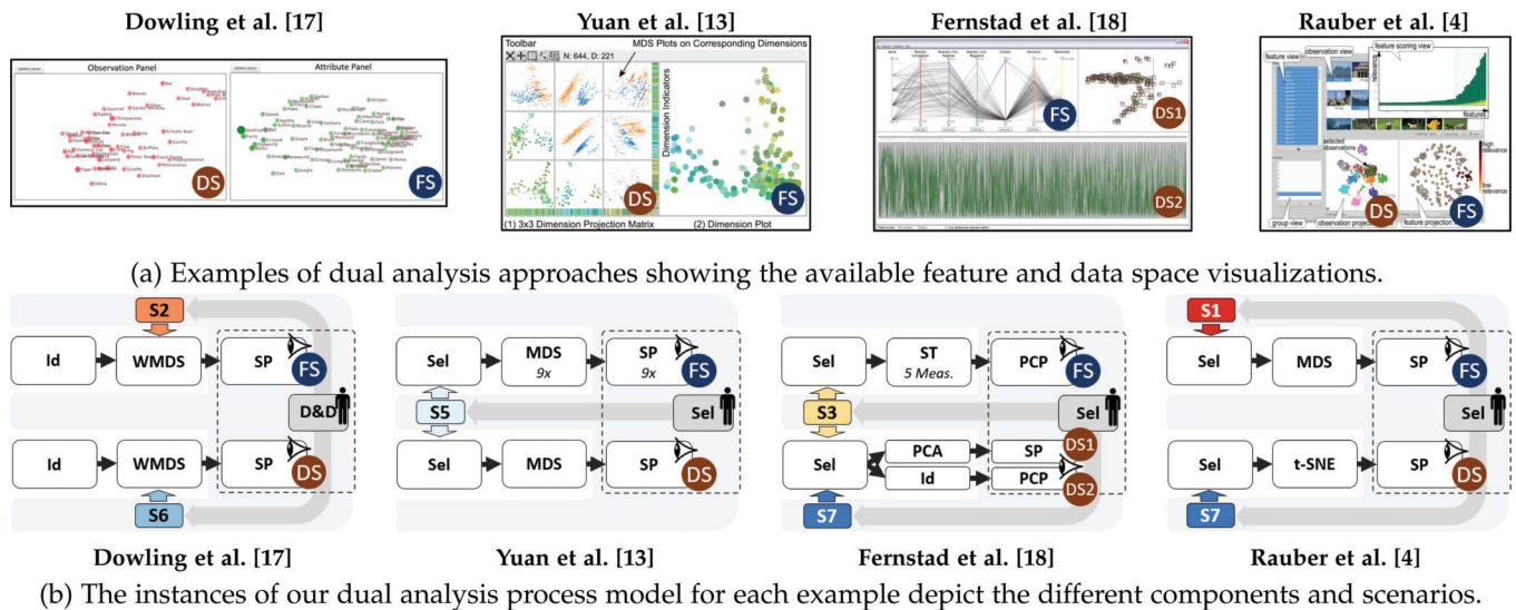
Fig. 6. We describe four approaches in Section VI-A to demonstrate that our dual analysis framework applies to existing approaches. We show the application of our model for the systems of Dowling et al. [17], Yuan et al. [13], Fernstad et al. [18], and Rauber et al. [4] as a representative set.
