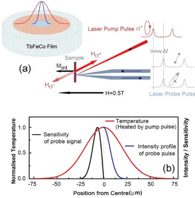
FIG. 1. (a) A schematic diagram of the experimental set-up with a bias field of H=0.5 T. H_{\sigma^+} represents the effective field of the pump pulse with \sigma^+ polarization (red line) due to the IFE. (b) The normalized radial sensitivity of Kerr rotation (only left half shown for clarity) and temperature distribution across the pump spot together with the intensity profile of the probe spot (only right half shown for clarity).
