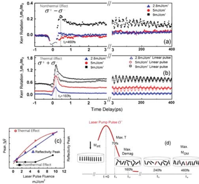
FIG. 3. (a) shows the difference between the \sigma^+ and \sigma^- pump pulses as a function of time. (b) The three solid curves show the sum of the \sigma^+ and \sigma^- pump pulses with time. The hollow curves are time domain responses excited by the linearly polarized laser pulse at the same pump fluences. (c) The peak amplitude of the thermal effect (red circles), of the reflectivity (blue triangles), and of the nonthermal effect (black squares) at a delay time of 460 fs as a function of the pump fluence. (d) shows a schematic diagram of the ultrafast process induced at a pump fluence of 9 \text{ mJ/cm}^2 .
