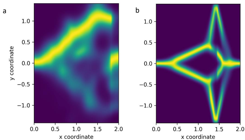
Figure 2. (a) Three-choice locust trajectories ( 45^\circ between posts) represented as heat map and (b) the respective simulation. Locusts showed a multi-bifurcation pattern when approaching three posts. The experimental trajectories are consistent with simulations according to Sridhar's model.
