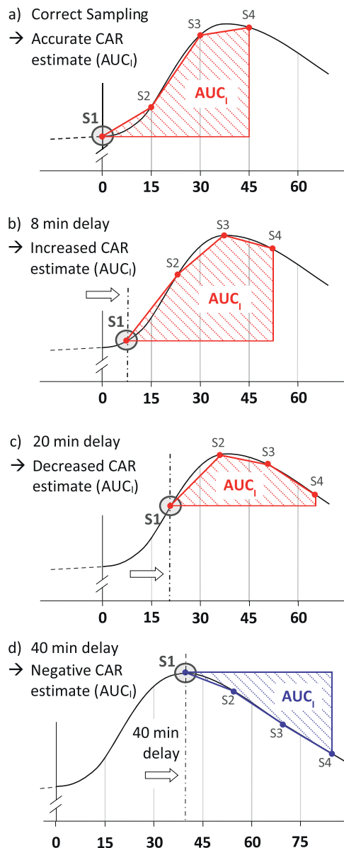
Fig. 3. Illustration of an exemplary CAR profile and the impact of delayed beginning of sampling after awakening on two common measures of post-awakening cortisol secretion, i.e., the first sample on awakening (S1) and the area under the curve with respect to increase (AUC I , Pruessner et al., 2003). The figure shows estimates given (a) correct sampling and for delays of (b) 8 min, (c) 20 min and (d) 40 min between awakening and collecting S1. Later samples (S2–S4) are shown to be collected in line with the specified 15 min intervals.
