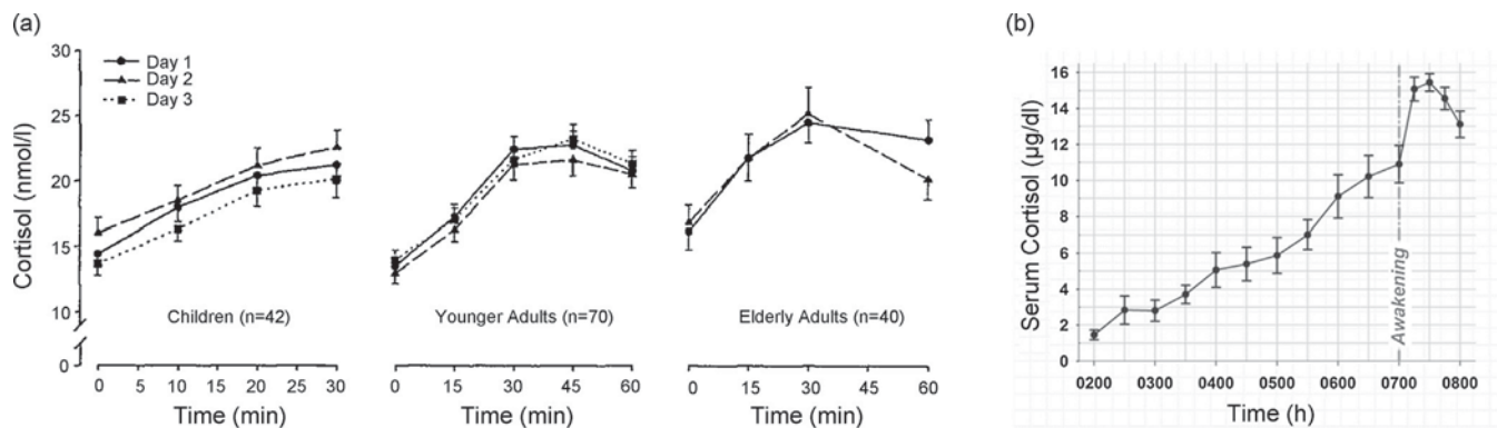
Fig. 2. (a) Mean ( \pm SEM) post-awakening cortisol values for three age groups from the first systematic description of the CAR (from Pruessner et al., 1997). (b) Sleep laboratory data showing the CAR to be superimposed on the pre-awakening cortisol increase (from Wilhelm et al., 2007). Both figures reproduced with permission.
