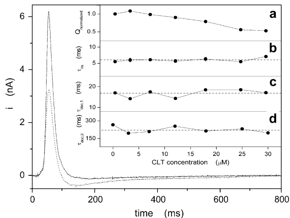
FIGURE 8 Experimental current transients obtained after a 100 \mu\text{M} ATP concentration jump in the absence ( solid line ) or presence ( dotted line ) of 25 \mu\text{M} CLT. The inset shows the dependence of the normalized charge ( a ) and time constants ( b , rising phase; c and d , decay phase) on CLT concentration. Dashed lines indicate averaged values for the time constants: ( b ) 6.0 \pm 0.6 ms; ( c ) 17 \pm 2 ms; and ( d ) 224 \pm 28 ms.
