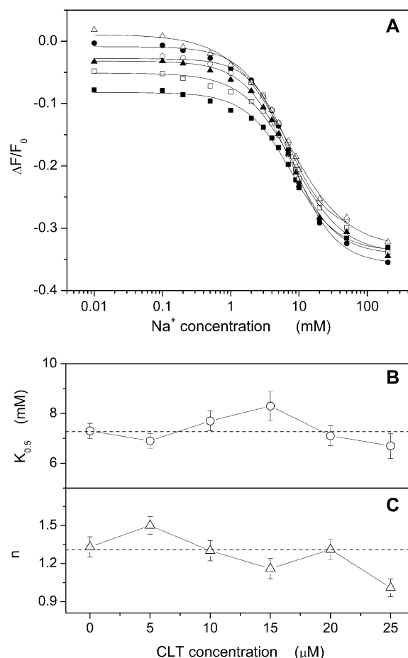
FIGURE 4 (A) Fluorescence changes correlated with titrations of the Na,K-ATPase by \text{Na}^+ ions in standard buffer at different CLT concentrations: 0 ( \bullet ), 5 ( \circ ), 10 ( \blacksquare ), 15 ( \square ), 20 ( \blacktriangle ), and 25 ( \triangle ) \mu\text{M} . For each titration the relative fitting curve obtained by a Hill function is shown. Panels B and C show the dependence on CLT concentration of the half-saturation constant and the Hill coefficient, respectively, for each fitting curve. Dotted lines mark the averaged values: 7.3 \pm 0.6 \text{ mM} for K_{0.5} and 1.3 \pm 0.2 for n .
