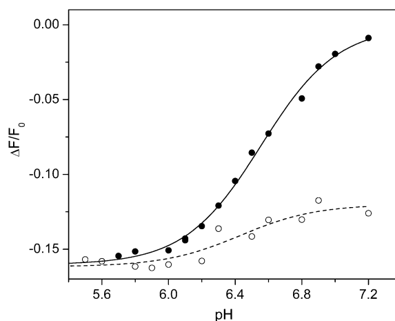
FIGURE 7 Fluorescence changes accompanying pH titration of Na,K-ATPase in standard buffer in the absence ( \bullet ) and presence ( \circ ) of 25 \mu\text{M} CLT. Drawn lines represent fitting curves of the experimental data by a Hill function: \text{pK} = 6.56 \pm 0.02 and n = 1.9 \pm 0.2 (solid line); \text{pK} = 6.4 \pm 0.1 and n = 1.9 (dotted line).
