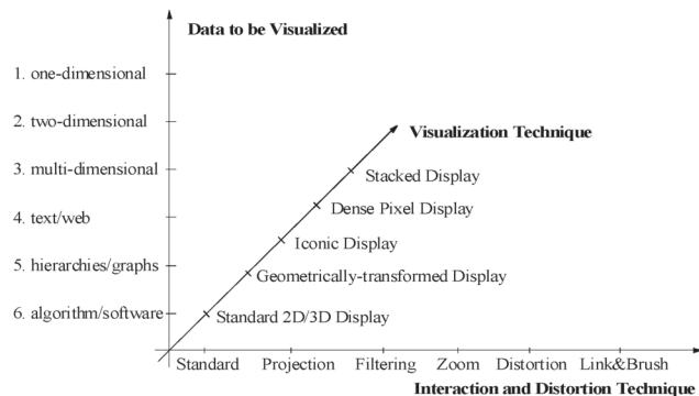
Fig. 1. Classification of Information Visualization Techniques
