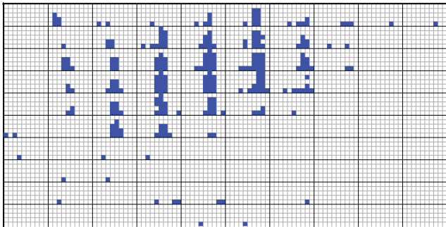
Fig. 5. Dimensional Stacking Visualization of Oil Mining Data (used by permission of M. Ward, Worcester Polytechnic ©IEEE)
