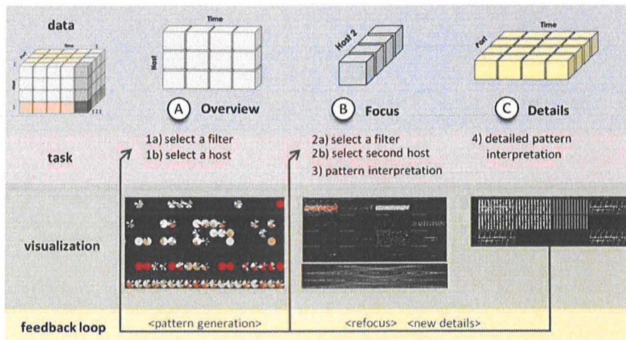
Figure 1: Analysis workflow with ClockView
