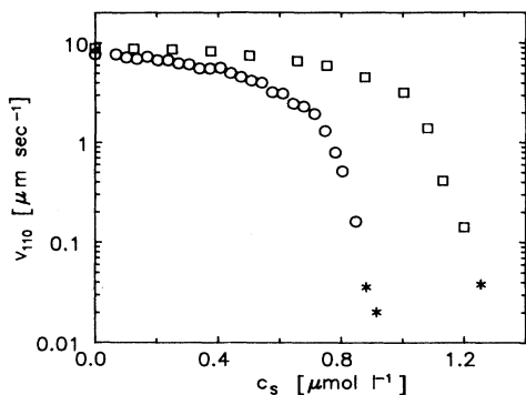
FIG. 6. The measured interfacial velocities v_{110} as a function of salt concentration, the circles are data on the A particles at the fixed volume fraction \Phi_A=0.003 and the squares are data on the B particles at \Phi_B=0.0022 . In both curves the stars denote points measured in the coexistence region.
