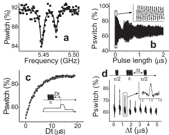
FIG. 3: (a) Qubit line shape at the optimal point. The solid line is a fit assuming a double Lorentzian shape. (b) Rabi oscillations (frequency 100\text{MHz} ) at the optimal point. The inset shows well-behaved oscillations with nearly no damping during the first 100\text{ns} . (c) Measurement of T_1 at the optimal point; the dashed grey line is an exponential fit of a time constant 4\mu\text{s} . (d) Spin-echo pulse sequence and signal at the optimal point.
