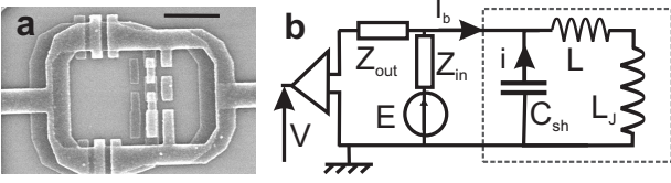
FIG. 1: (a) SEM picture of the sample. The flux qubit is the small loop containing four Josephson junctions in a row ; the SQUID is constituted by the outer loop containing the two large junctions. The bar equals 1\mu\text{m} . (b) Measuring circuit diagram. The SQUID, represented by its Josephson inductance L_J , is shunted by an on-chip capacitor C_{sh} through superconducting lines of inductance L , forming the plasma mode.
