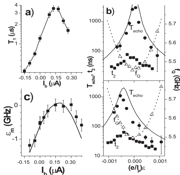
FIG. 4: (a) Measurement of T_1 versus I_b at the flux-noise insensitive point \epsilon = 0 . (b) Measurement of T_{echo} (circles), t_2 (squares) and of the qubit frequency (triangles), as a function of \epsilon for I_b = I_b^* (top) and I_b = 0 \mu A (bottom). The dotted line is a fit to the formula for \nu_q ; the solid black line is the prediction of equation 1 for T = 70mK and Q = 150 . (c) Value of \epsilon for which t_2 is maximum (full squares) compared to the theoretical \epsilon_m(I_b) (full line).
