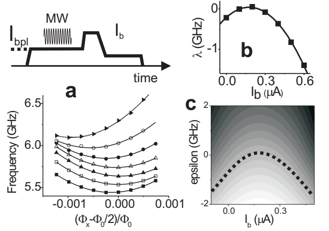
FIG. 2: (a) Top : Principle of the spectroscopy experiments : a bias current pulse of amplitude I_{bpl} < I_C \sim 1\mu A is applied while a microwave pulse (MW) probes the qubit resonance frequency. The qubit state is finally measured by a short bias current pulse as discussed in [3]. Bottom : Qubit spectroscopy for I_{bpl} varying between 0\mu A to 0.6\mu A with steps of 0.1\mu A (bottom to top). The curves were offset by 100MHz for clarity. The solid curves are fits to the formula for \nu_q . (b) Curve \lambda(I_b) deduced from the spectroscopy curves as explained in the text. The solid line is a parabolic fit to the data. The decoupling condition is satisfied at I_b^* = 180 \pm 20nA . (c) Calculated frequency shift \delta\nu_0(I_b, \epsilon) for the parameters of our sample. The white scale corresponds to -20MHz , the black to +40MHz . Along the dotted line \epsilon_m(I_b) , \delta\nu_0 = 0 .
