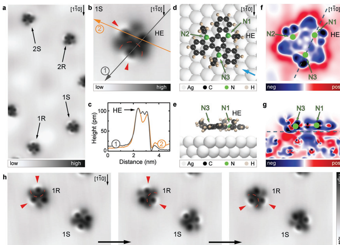
Figure 1. TAT molecules on Ag(111). a) Large-scale STM image of TAT molecules on Ag(111) ( U = 10 mV, I = 100 pA, 9 \times 18 nm 2 ). b) STM image of a single TAT molecule (1S-type) ( U = 10 mV, I = 100 pA, 3 \times 3 nm 2 ). The highest ethyl group is marked as HE. Depressions localized close to the other ethyl groups are denoted by red triangles and the boomerang-shaped feature within the molecule by a dashed red semicircle. c) Height profiles along the gray and orange lines shown in (b). d) Optimized adsorption geometry of TAT on Ag(111) (1S-type). The theoretical studies suggest that TAT molecules adsorb on atop sites, meaning that the central benzene ring is located above a Ag atom. This can be further specified into atop-fcc (pyrrole above fcc-hollow sites) and atop-hcp adsorption sites (pyrrole above hcp-hollow sites), referred to as 1 and 2. Additionally, the presence of the surface leads to two non-superimposable configurations of the TAT molecule labeled as R and S. Four possible adsorption types—1R, 1S, 2R, and 2S—are indicated by arrows in (a). e) Side view of the DFT-optimized adsorption geometry along the view direction marked by a blue arrow in (d). f,g) Charge-density difference calculated as \Delta\rho(\mathbf{r}) = \rho_{\text{TAT}/\text{Ag}}(\mathbf{r}) - \rho_{\text{Ag}}(\mathbf{r}) - \rho_{\text{TAT}}(\mathbf{r}) and plotted in units of e \text{ nm}^{-3} for geometry (d) and (e), respectively. Signs are chosen such that a positive charge or missing electrons are counted as positive. The color scale ranges from -4 e \text{ nm}^{-3} (blue) to 4 e \text{ nm}^{-3} (red), where e = |e| is the elementary charge. Cut plane positions are marked by blue dashed lines in (f) and (g). h) A series of subsequently recorded STM images showing switching between three equivalent bonding configurations within their adsorption types—1R and 1S ( U = 10 mV, I = 100 pA, 7 \times 5 nm 2 ). Characteristic molecular features are highlighted by red triangles and dashed red semicircles.
