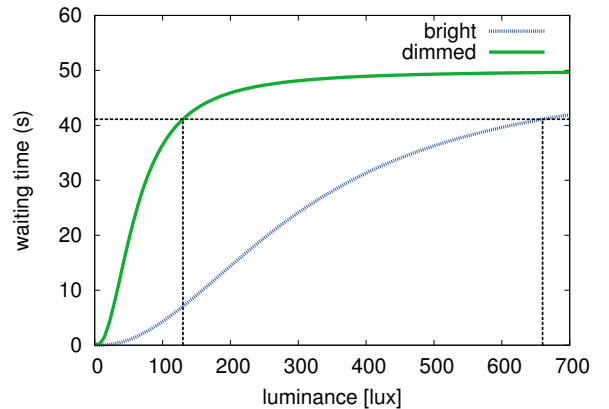
Figure 4: Mapping of luminance values to waiting time (equations 1 and 2) for two light settings: bright and dimmed (black lines indicate maximal luminance values and w_{\max} is 50 seconds).
