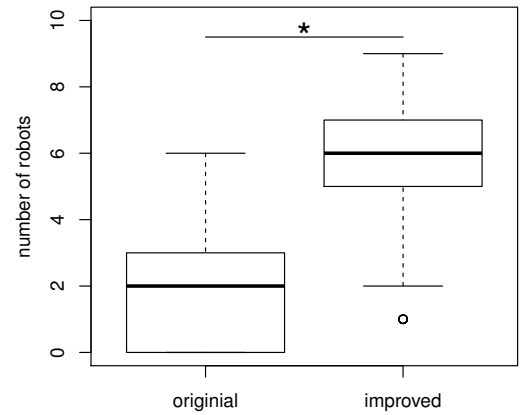
Figure 8: Comparison between the performance of both BEECLUST implementations in terms of the number of stopped robots in zone I during the last ten minutes time interval in the one dimmed light experiments.
