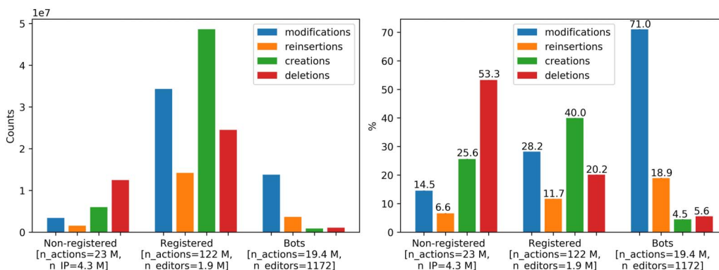
Figure 8. Distribution of actions performed by each type of editors. The left plot shows the total actions (y-axis) per type of account (x-axis), and type of action (legend). The right plot shows the percentage (y-axis) of the type of actions (legend) within the account type (x-axis). The x-axis also presents the total number of actions (n_actions) and editors or IP addresses (n_editors or n_IP) for each account type.
