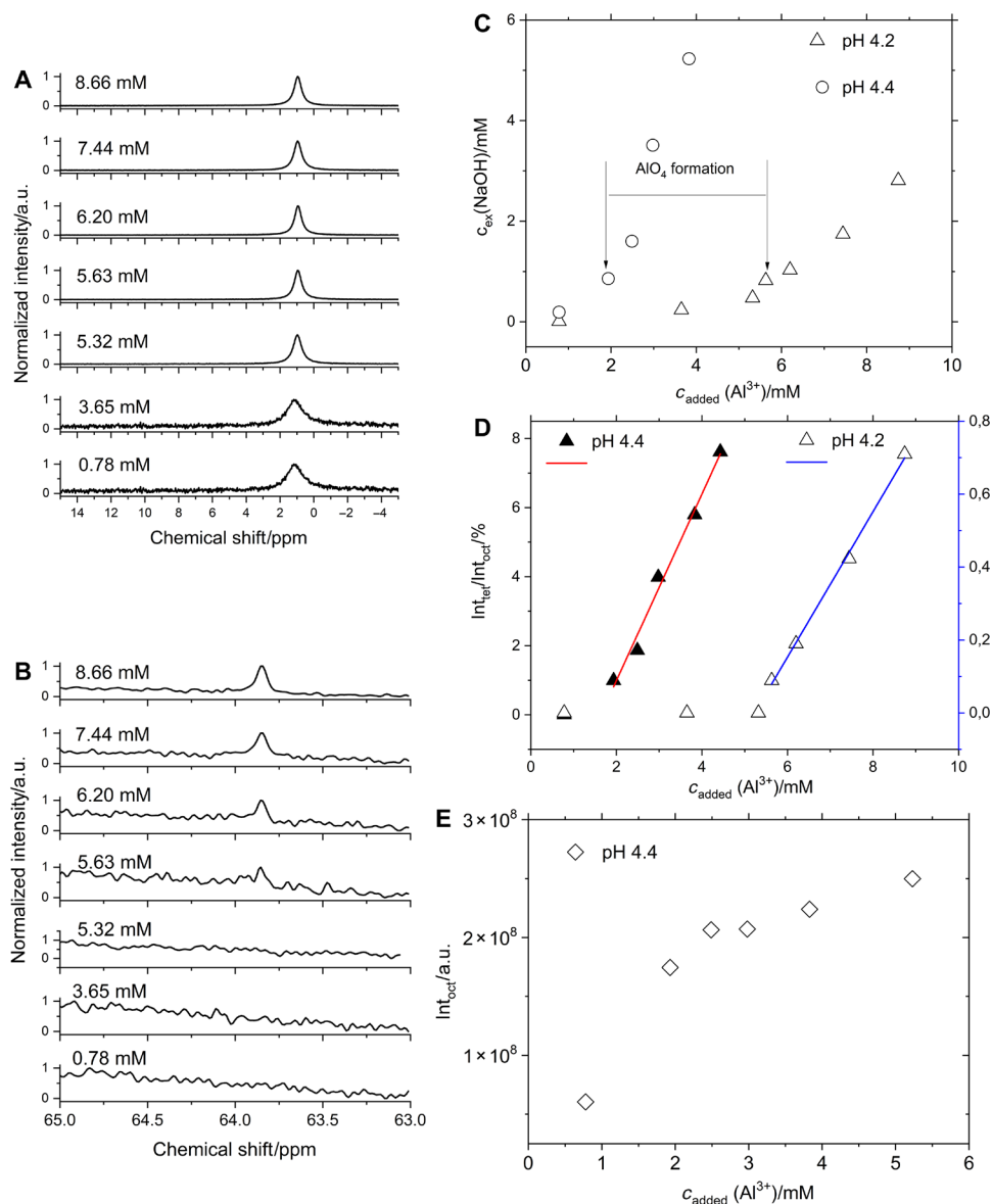
Fig. 4. Influence of concentration on Al(III) speciation during the early stages of nucleation. ^{27}\text{Al} -NMR spectra of samples drawn at specific total Al(III) concentrations as indicated in the graphs during titration experiments: (A) Resonance for the monomeric species and (B) for the \text{AlO}_4 environment at different Al(III) concentrations at pH 4.2. In combination with the titration curves (Fig. 1A) and stop experiments (Fig. 1B), this shows that tetrahedral environments emerge after nucleation. (C) Sampling points at pH 4.2 and 4.4 with indicated concentration of \text{AlO}_4 from NMR, confirming its appearance after the change in hydrolysis regime, i.e., after phase separation. (D) Evolution of the amount of tetrahedral \text{AlO}_4 species given as a percentage of the octahedral population ( \text{Int}_{\text{tet}}/\text{Int}_{\text{oct}} ) assessed from the intensity of integrated NMR peaks, showing a linear increase with Al(III) addition at both pH values. (E) Resonance intensity due to octahedral Al(III) versus the total [\text{Al}^{3+}] concentration. The amount continues to increase after \text{AlO}_4 formation at 1.93 mM [\text{Al}^{3+}] but with an altered slope, implying the existence of an intermediate dynamic (meta)stable state between octahedral and tetrahedral species.
