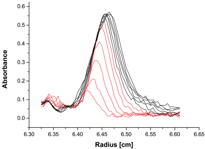
Fig. 2 Experimental radial absorption scans at 450 nm after the NaBH 4 solution was overlaid over the AgNO 3 solution. A slight movement of the reaction boundary towards the cell bottom can be observed as a result of the ca. 2-times faster BH 4 - diffusion as compared to Ag + . 51,52
