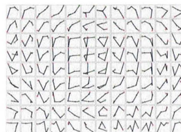
(b) Self-Organizing Trajectory Map
