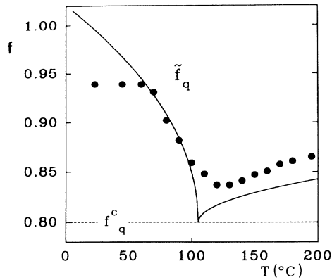
FIG. 7. The effective Debye-Waller factor \tilde{f}_q at q_0 defined by the inflection point t_i of the G(t) vs \log_{10}(t) curves, i.e., \tilde{f}_q = h_q G(t_i) . The solid circles are determined from the parameters of Fig. 2 and f_q^c = 0.80 . The solid lines are the square-root asymptotes of the formula (4.4) law scaled with h_q(T) = h_q(T_c) and the linear fit for \sigma(T) from Fig. 2(a).
