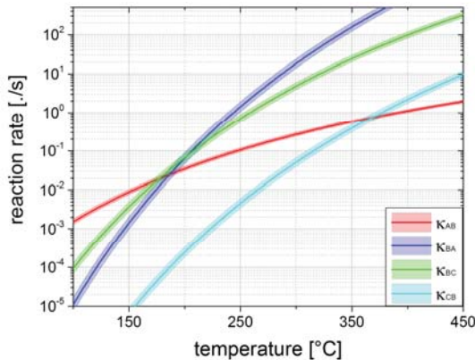
Figure 2: Calculated reaction rates versus temperature. Colored areas depict the uncertainty.
