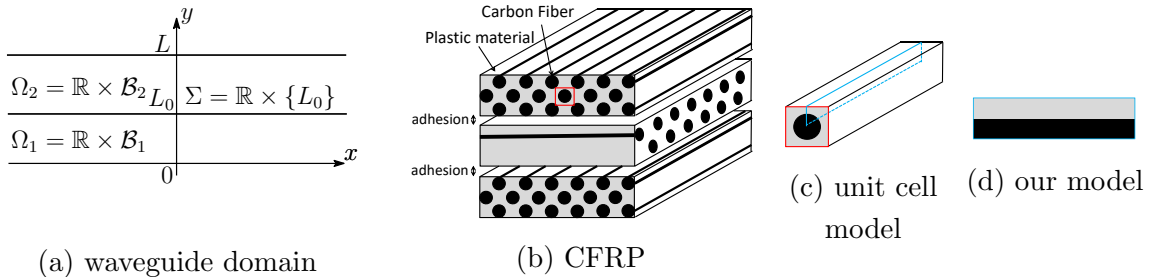
Figure 1: waveguide domain, standard product of CFRP, unit cell model and our model
