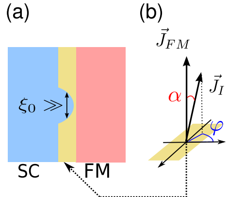
FIG. 2: (Color online) (a) The Andreev point contact with spin-active interface (b) Interface with FM exchange field \vec{J}_{FM} , \alpha and \varphi characterize the orientation of \vec{J}_I with respect to \vec{J}_{FM} . The dashed arrow indicates the area where the misaligned interface magnetic moment resides.
