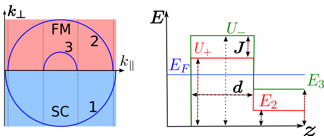
FIG. 3: (Color online) Sketch of the box-potential model that we consider in this section (right) and of the corresponding Fermi-surface geometry (left). The model parameters are indicated.
