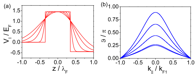
FIG. 10: (Color online) (a) Shape function of the scattering potential (average between both spin directions) for \sigma = 0 \dots 0.7 \lambda_F and \sigma + d = 0.7 \lambda_F . E_2 = -0.1 E_F and E_3 = -0.8 E_F . (b) The spin-mixing angle \vartheta as a function of impact angle for the different potentials plotted in (a). \sigma increases from bottom to top.
