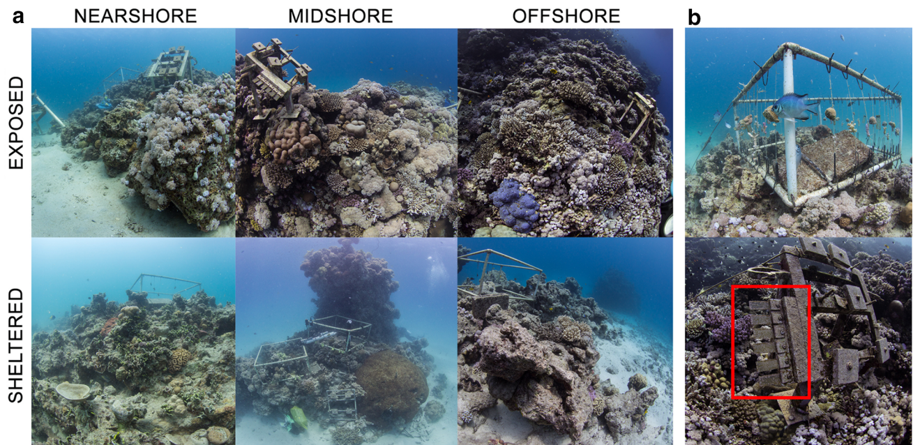
Fig. 2 Study sites and in situ setup of moored frames. a The study sites along the cross-shelf gradient, which represent reefs ranging from exposed fore-reef well-mixed habitats to turbid back-reef
