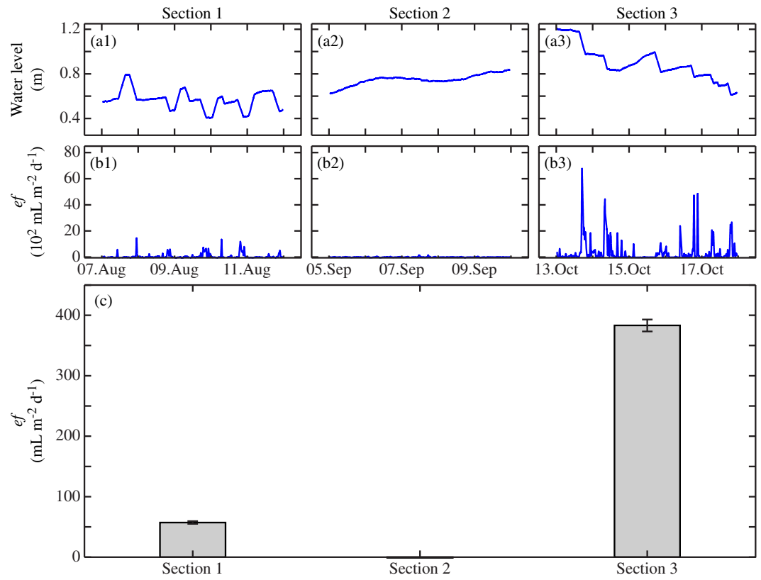
Figure 5. Water level (a) and ebullition flux (b) dynamics and average ebullition flux (c) during the three specific time sections representing the three different modes of operation (1) diurnal pumping and turbination, (2) no pumping and no turbination, and (3) diurnal turbination. The water level is relative to the reference water level of 658.5 m a.s.l.
