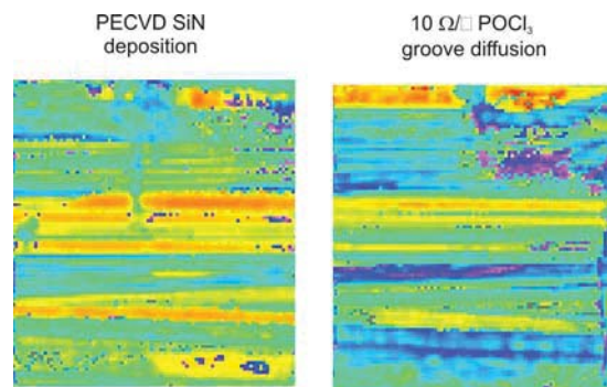
Figure 6: Degradation after heavy diffusion. Effusion of hydrogen.
