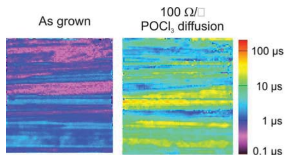
Figure 4: Lifetime map of as grown wafer on the left. Improvement after 100 Ohm/sq \text{POCl}_3 diffusion (P-gettering).
