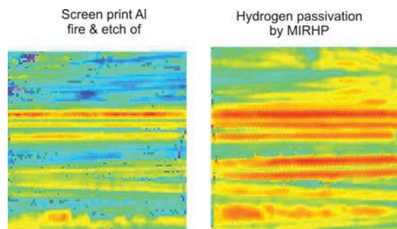
Figure 8: Improvement of hydrogen passivation by MIRHP.
