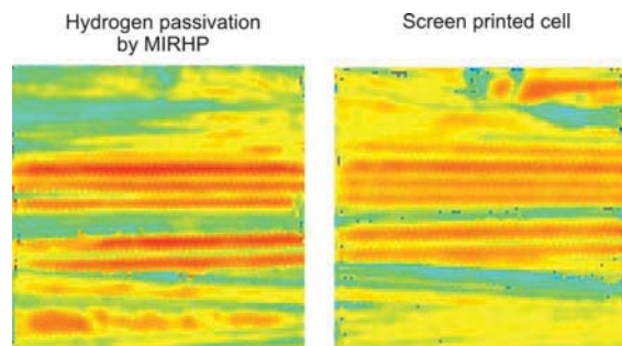
Figure 9: Comparison of lifetime maps. Buried contact process (left) to screen printing process (right).
