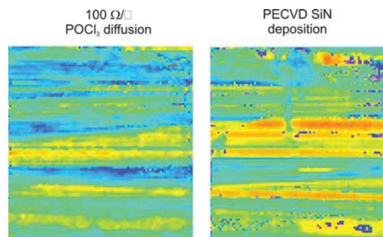
Figure 5: Improvement by PECVD-SiN deposition only. No firing step was applied.
