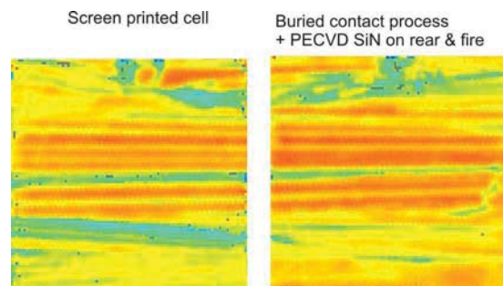
Figure 10: Alternative hydrogen passivation.
