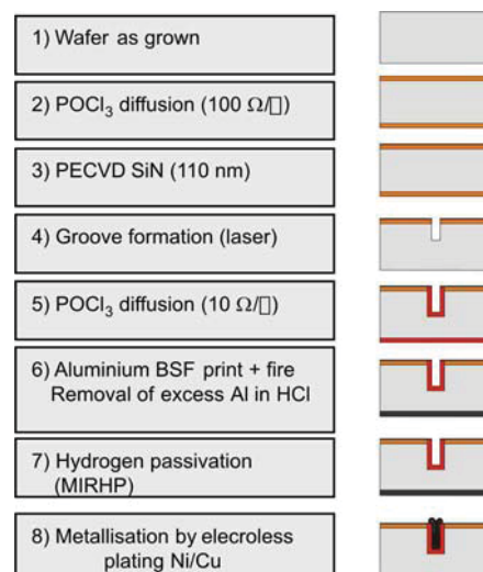
Figure 2: Buried contact process sequence with String Ribbon silicon.
